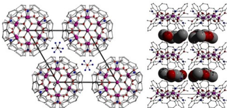
Figure 3. (left) Packing observed in [\text{Co}(\text{II})_7(\text{OH})_6(\text{L}_1)_6](\text{NO}_3)_2 ( 1 ) as viewed down the c axis of the unit cell, highlighting the 1D columns observed in 1 (and 2 ). (right) Crystal packing observed in [(\text{MeOH})_2\text{C-Co}(\text{II})_7(\text{OH})_6(\text{L}_1)_6](\text{NO}_3)_2 ( 2 ). The MeOH guests are space-fill represented.
