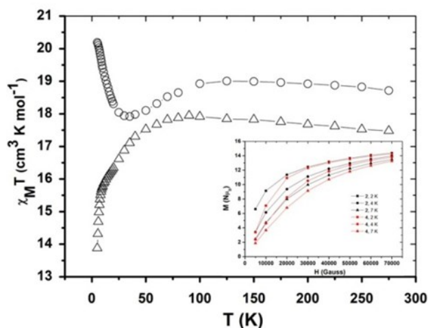
Figure 10. Plots of \chi_M T vs. T obtained from polycrystalline samples of 2 (o) and 4 ( \Delta ) respectively measured in an applied field of 0.1 T and 5-300 K temperature range. Solid lines are for visual purposes only. (inset) Plots of M/N\mu_B vs H (G) data obtained from 2 (black) and 4 (red) at three different temperatures (2, 4 and 7 K) in an 0.5-7 T applied magnetic field sweep.
