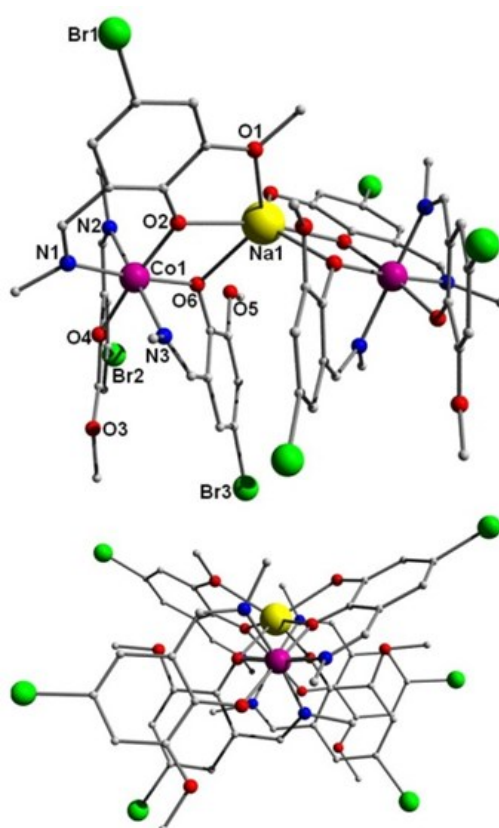
Figure 8. Crystal structures of [\text{Co(III)}_2\text{Na(I)}_1(\text{immp-Br})_6](\text{BF}_4) ( 6 ) as viewed perpendicular (top) and parallel (bottom) to the V-shaped plane of the molecule. Colour code: Purple (Co), Yellow (Na), Red (O), Blue (N), Green (Br) and Grey (C). H-atoms omitted for clarity.
