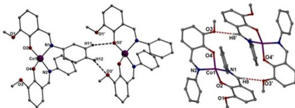
Figure 7. Crystal structure of [\text{Co(II)(L}_2)_2] ( 5 ) highlighting the close proximity of neighbouring monomers within the H-bonded chains (left) and between the chains (right). H-bonding shown using dashed lines.
