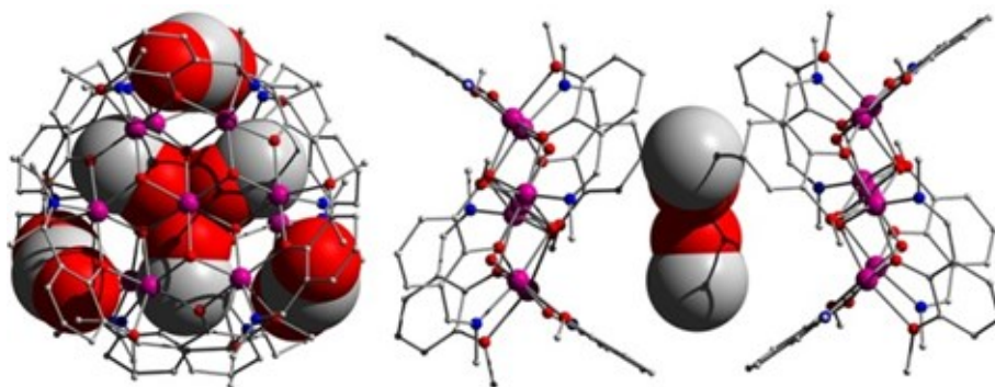
Figure 2. Space-filled representations of the two crystallographically unique guest MeOH molecules lying within the molecular cavities formed by two double-bowl [\text{Co}(\text{II})_7] units in complex 2 .
