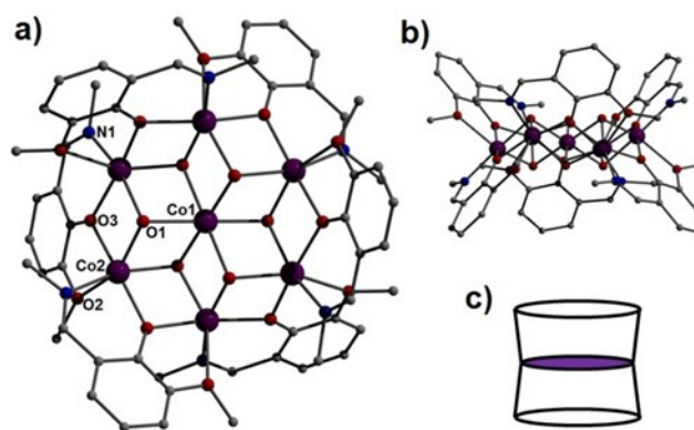
Figure 1. (a) Crystal structure of 1 as viewed perpendicular (a) and parallel (b) to the planar {Co(II) 7 } core. (c) Schematic representation of the double-bowl topology in 1 and its analogues. Colour code (used throughout this work): Purple (Co), Red (O), Blue (N), Grey (C). H-atoms omitted for clarity.
