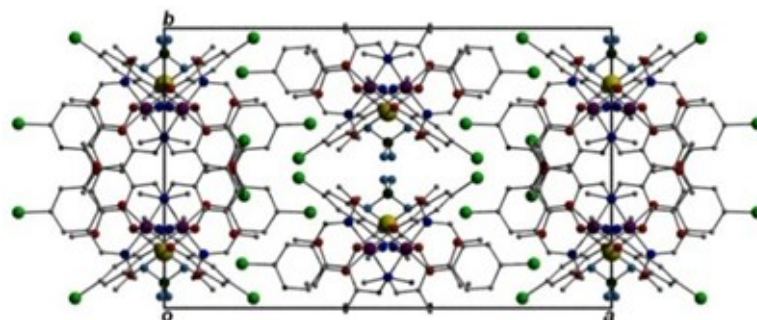
Figure 9. Crystal packing observed in 6 as viewed along the c axis. hydrogen atoms omitted for clarity. Colour code: Yellow (Na), Purple (Co), Red (O), Dark Blue (N), Grey (C), Green (Br), Dark Green (B), Light Blue (F).
