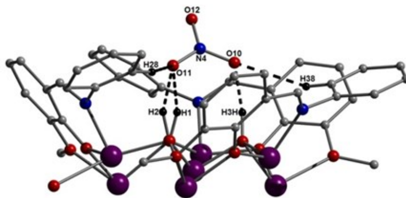
Figure 5. View of a \text{NO}_3^- anion occupying one half of a double-bowl [\text{Co(III)Co(II)}_6] unit in 4 . Intermolecular interactions between the host and guest are represented as dashed lines. Actual distances are given in the main text.
