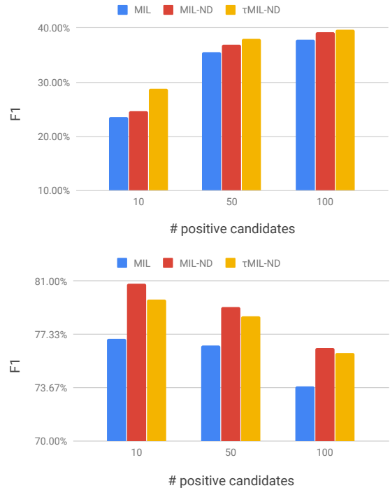
Figure 4: F1 (top: ‘All’; bottom: ‘In E^+ ’) on the development set with different numbers of positive candidates.
