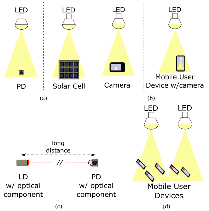
Fig. 1. Different OWC technologies. (a) VLC system with a PD (left) and a solar cell (right). (b) OCC system with a camera with a lens and image sensor (left) and a mobile user device with an embedded camera with a lens and image sensor (right). (c) FSO communication system with an LD and PD. (d) LiFi system with multiple LEDs and mobile user devices.
