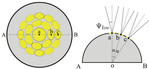
Fig. 3. An angular diversity receiver is constructed by assembling multiple small photo-detectors on a semi-spherical base.
