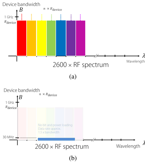
Fig. 4. The potential of the combined infrared spectrum and visible light spectrum: (a) Device bandwidth has to be large to correspond to the spectral emission profile of the devices, and with WDM it would be possible to leverage the potential of the huge optical spectrum; (b) off-the-shelf white LEDs typically are single devices emitting a broad spectrum using phosphor based colour converting materials. This limits device bandwidth and prevents the significant WDM gains. Therefore, those systems completely rely on techniques that most effectively utilize the available bandwidth such as bit-and-power loading.
