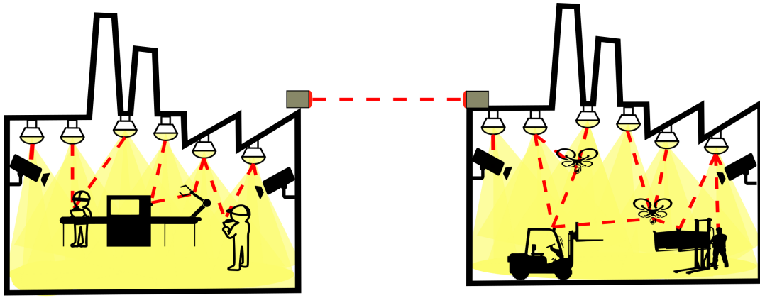
Fig. 2. Illustration of the indoor and outdoor OWC technologies for an industrial private network. The optical links are shown by red dashed lines.
