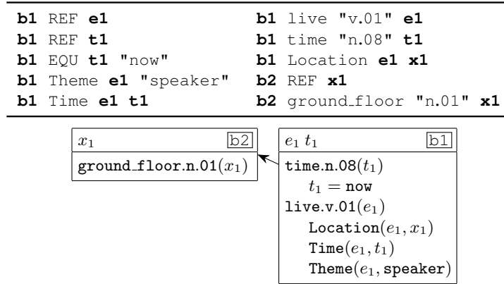
Figure 1: The clause representations (top) and box-style representations (bottom) for the sentence I live on the ground floor.
