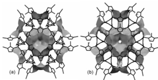
Figure 3. Packing arrangement of ZIF-8 at (a) ambient pressure and (b) ZIF-8-II at 1.47 GPa. ZnN4 tetrahedron are drawn as rigid polyhedra. H-atoms have been excluded for clarity. Note the change in orientation of the imidazolate groups on undergoing the transition from (a) to (b).
