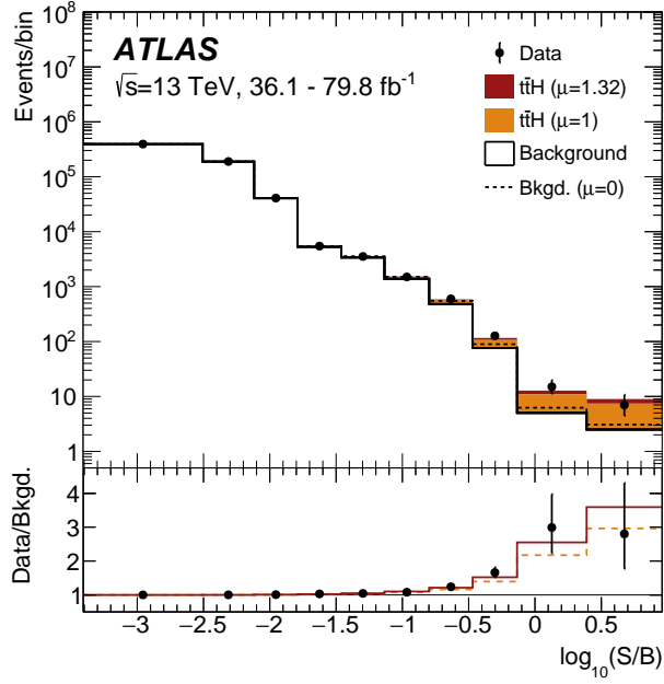
Figure 4: Observed event yields in all analysis categories in up to 79.8 \text{ fb}^{-1} of 13 \text{ TeV} data. The background yields correspond to the observed fit results, and the signal yields are shown for both the observed results ( \mu = 1.32 ) and the SM prediction ( \mu = 1 ). The discriminant bins in all categories are ranked by \log_{10}(S/B) , where S is the signal yield and B the background yield extracted from the fit with freely floating signal, and combined such that \log_{10}(S + B) decreases approximately linearly. For the H \rightarrow \gamma\gamma analysis, only events in the smallest m_{\gamma\gamma} window containing 90% of the expected signal are considered. The lower panel shows the ratio of the data to the background estimated from the fit with freely floating signal, compared to the expected distribution including the signal assuming \mu = 1.32 (full red) and \mu = 1 (dashed orange). The error bars on the data are statistical.
