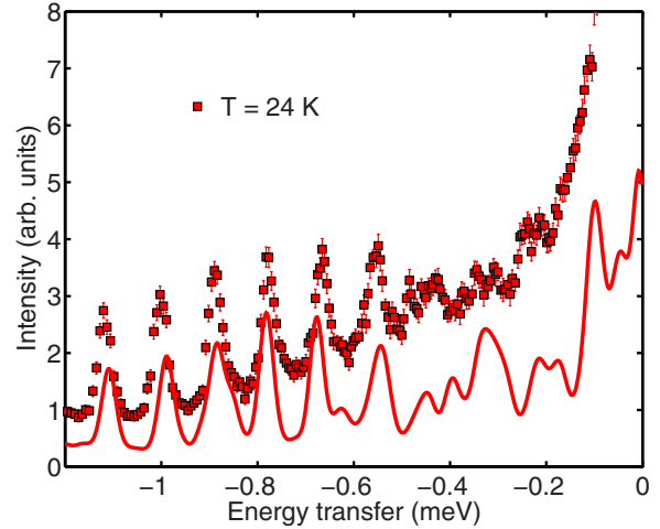
FIG. 11. (Color online) High-resolution INS spectra of molecule (3) collected on IN5 with incident wavelength 10.5 Å at 24 K. The energy gain spectra is displayed. Continuous lines are the calculations using the spin Hamiltonian of Eq. (2).
