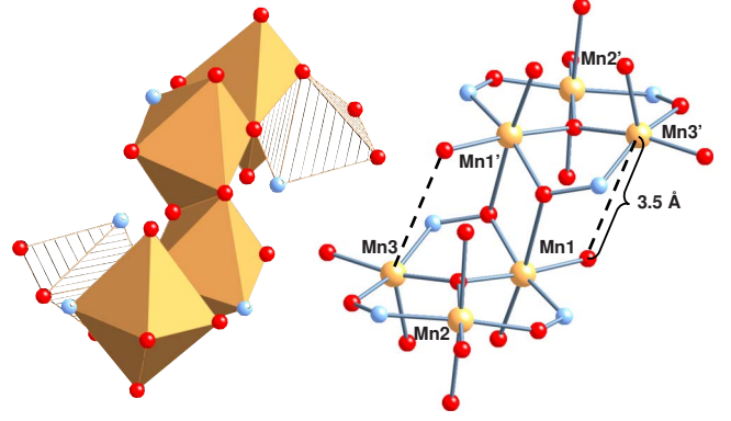
FIG. 2. (Color online) Structure of the Mn 6 (1) molecular core. The Mn 3+ ions are located at the vertices of two oxocentered triangles. Ions Mn1, Mn2, Mn1', and Mn2' are in octahedral geometry and ions Mn3 and Mn3' in square pyramidal geometry, as highlighted in filled and striped orange (left figure). Color scheme: Mn, large orange circles; O, dark red circles; and N, small light blue circles. H and C ions are omitted for clarity.
