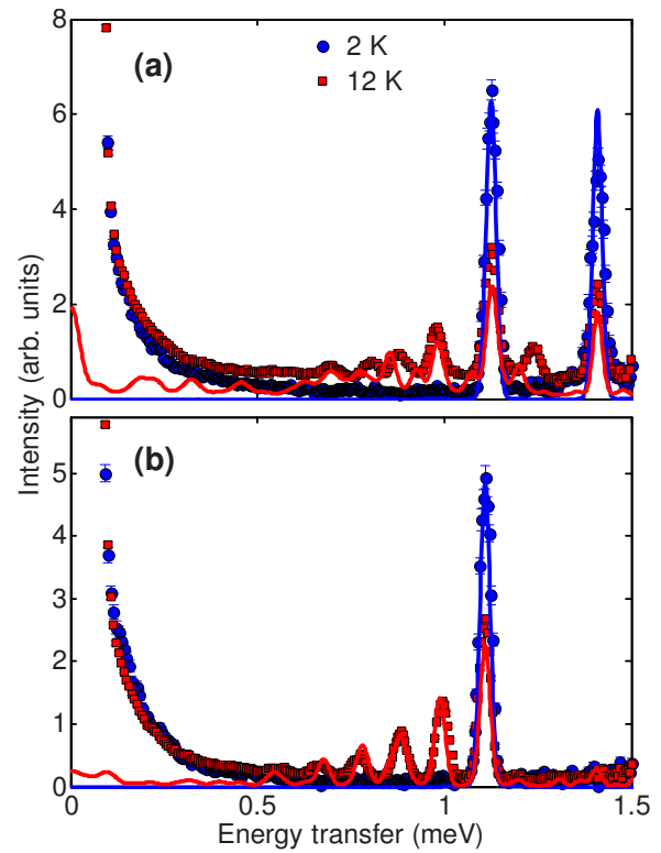
FIG. 9. (Color online) INS spectra collected on IN5 with incident wavelength of 6.7 \text{\AA} at T=2 K (blue circles) and T=12 K (red squares). (a) for sample (2) and (b) for sample (3). The spectra calculated with the parameters listed in Table II are shown as continuous lines.
