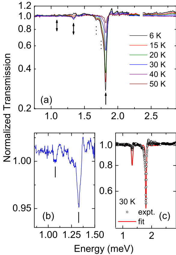
FIG. 3. (Color online) (a) FDMR spectra of unpressed polycrystalline powder of (1) recorded at various temperatures. The intensity of the higher-frequency resonance line decreases with temperature while that of the lower-frequency lines increases up to 30 K, beyond which it decreases again. Dotted lines indicate resonance lines due to impurities. (b) Expanded view of the low-frequency part of the 30 K spectrum. (c) Experimental and fitted spectrum at T = 30 K using the GSH approximation. Note the logarithmic scale in (a) and (c).
