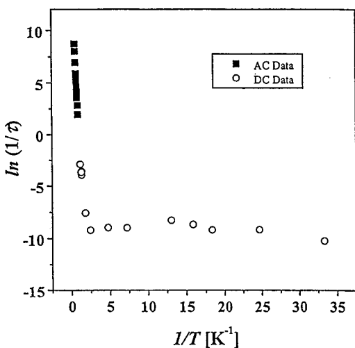
FIG. 2. Plot of the natural logarithm of the relaxation rate ( 1/\tau ) vs the inverse absolute temperature for complex 4. The symbol (■) represents the data collected with the ac magnetic susceptibility technique, and the magnetization decay data are indicated by the symbol (○).
