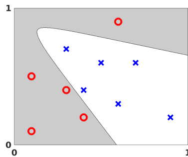
FIG. 6.3. Visualization of output from an artificial neural network applied to the data in Figure 2.1 with an additional data point. Here we trained the network using the stochastic gradient method with back propagation. The same optimization problem was solved with the lsqnonlin routine from MATLAB in order to produce Figure 2.5.
