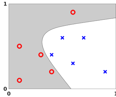
FIG. 6.2. Visualization of output from an artificial neural network applied to the data in Figure 2.1. Here we trained the network using the stochastic gradient method with back propagation—behaviour of cost function is shown in Figure 6.1. The same optimization problem was solved with the lsqnonlin routine from MATLAB in order to produce Figure 2.4.
