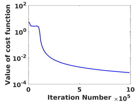
FIG. 6.1. Vertical axis shows a scaled value of the cost function (2.6). Horizontal axis shows the iteration number. Here we used the stochastic gradient method to train a network of the form shown in Figure 2.3 on the data in Figure 2.1. The resulting classification function is illustrated in Figure 6.2.
