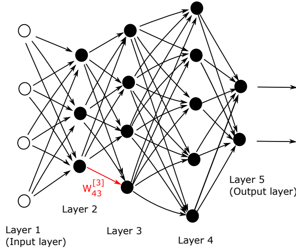
FIG. 3.1. A network with five layers. The edge corresponding to the weight w_{43}^{[3]} is highlighted. The output from neuron number 3 at layer 2 is weighted by the factor w_{43}^{[3]} when it is fed into neuron number 4 at layer 3.
