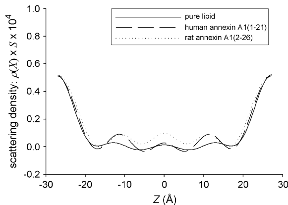
FIGURE 6 Water distribution profiles of DMPC/DMPS (3:1 molar ratio) in the absence (solid line) and presence of human annexin A1(1-21) (dashed line) and rat annexin A1(2-26) (dotted line).
