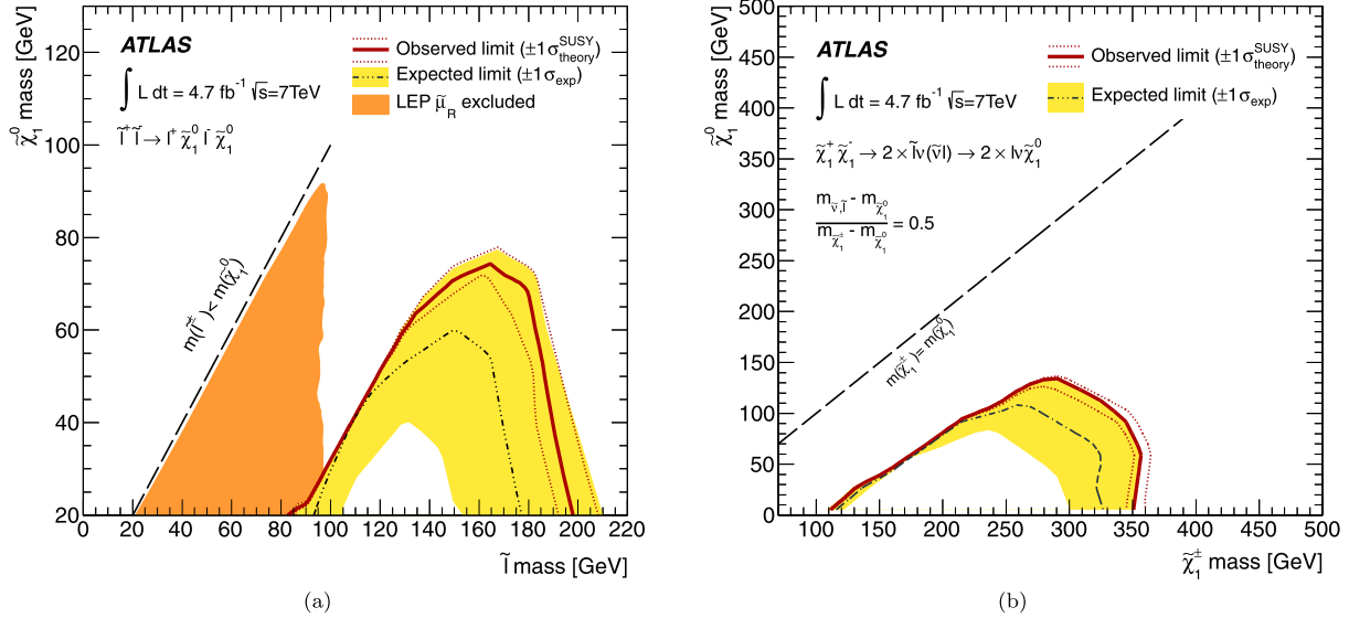
Fig. 2. 95% CL exclusion limits for \tilde{t}\bar{\tilde{t}} pair production in the m_{\tilde{\ell}}-m_{\tilde{\chi}_1^0} mass plane of (a) the direct slepton pMSSM and (b) \tilde{\chi}_1^\pm\tilde{\chi}_1^\mp pair production in the simplified model. The dashed and solid lines show the 95% CL s expected and observed limits, respectively, including all uncertainties except for the theoretical signal cross-section uncertainty (PDF and scale). The solid band around the expected limit shows the \pm 1\sigma result where all uncertainties, except those on the signal cross-sections, are considered. The \pm 1\sigma lines around the observed limit represent the results obtained when moving the nominal signal cross-section up or down by the \pm 1\sigma theoretical uncertainty. Illustrated also in (a) is the LEP limit [28] on the mass of the right-handed smuon, \tilde{\mu}_R . The LEP limit is a conservative limit on slepton pair production: if right-handed slepton masses are excluded, left-handed sleptons of equivalent masses are automatically excluded. (For interpretation of the references to colour, the reader is referred to the web version of this Letter.)
