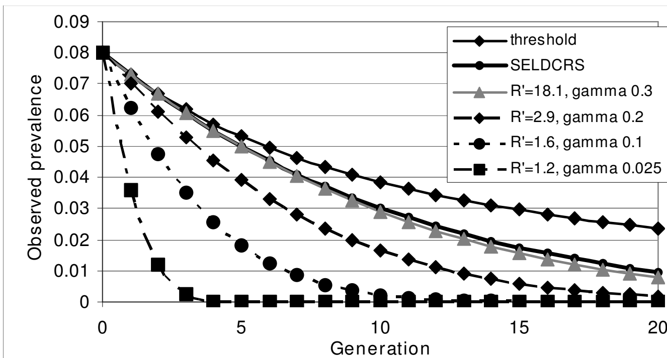
Figure 2 Predicted response to selection for resistance to footrot depending on the model used, the notional reproductive rate R' and the initial recovery rate \gamma . Selection is on \gamma , with \lambda = 0.0333 , \nu = 0.1667 , p^* = 0.08 and h^2 = 0.3 .
