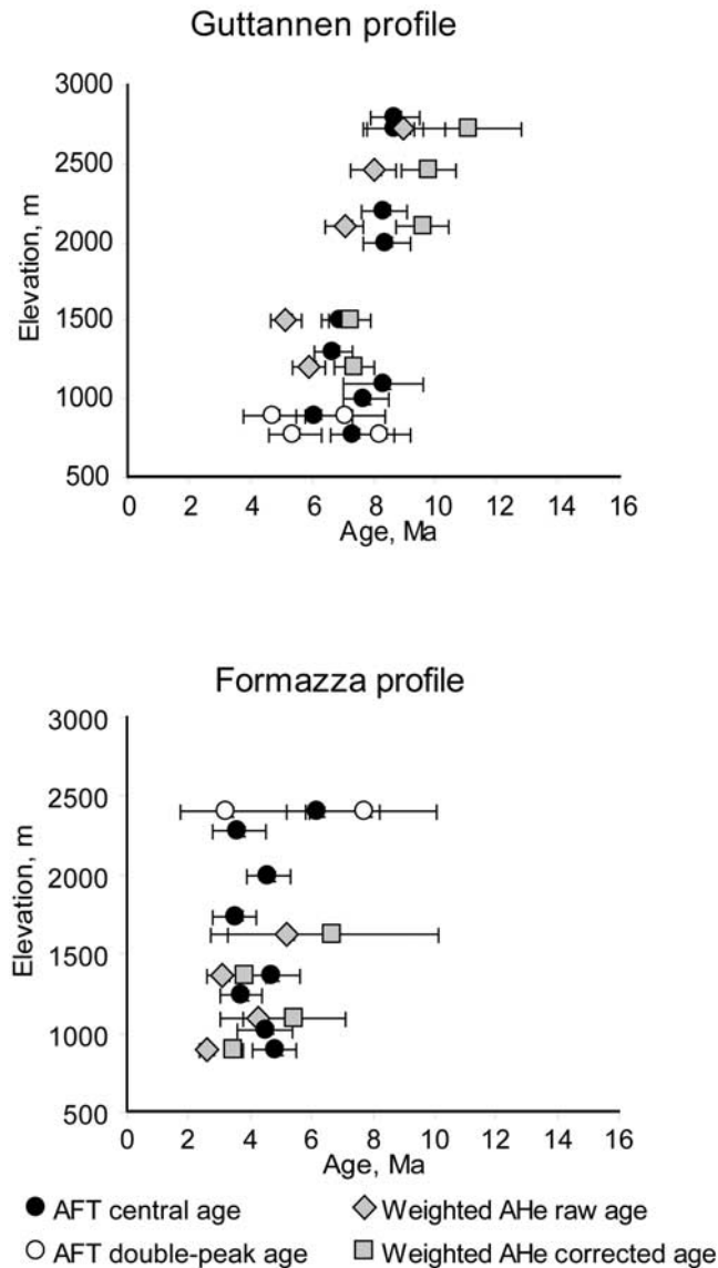
Figure 7. Comparison of AFT ages (circles, 1\sigma error bars) with uncorrected (diamonds) and alpha-ejection-corrected (squares) 1\sigma analytical uncertainty-weighted average AHe ages (with error bars as explained in Table 3), obtained in the Guttannen and the Formazza elevation profiles. White circles are used in addition to the black symbols showing central age, in samples where single-grain AFT ages are dispersed and can be characterized as belonging to several age populations, each grouping at least 30% of dated grains.
