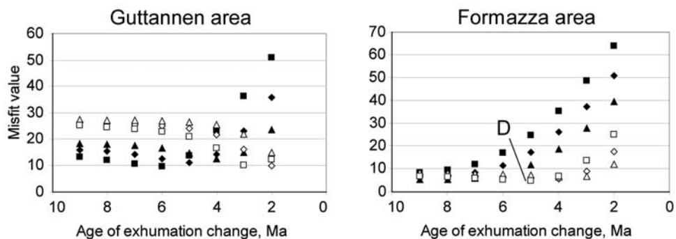
Figure 14. Cumulated misfit between predicted and measured AFT and AHe ages in the Guttannen and the Formazza study areas for different scenarios of single-step exhumation rate increase occurring at the age indicated on the x axis, with different intensities (200 to 700 m/Ma in black, or 300 to 1000 m/Ma in white) and a choice of relief variation. Diamonds, steady relief; squares, relief reduction from \beta = 1.3 to 1; triangles, relief increase from \beta = 0.7 to 1. See text for further details on the method. D ( \mu = 4.8 ) refers to case D in Figure 15.
