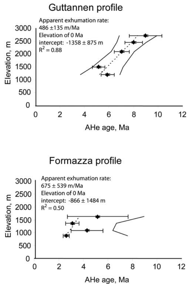
Figure 6. AHe age-elevation profiles and weighted regression relationship (dashed line, regression line; bold lines, 95% confidence interval) for the Guttannen and the Formazza areas. Weighted-average-uncorrected AHe ages were used, with error bars as explained in Table 3.
