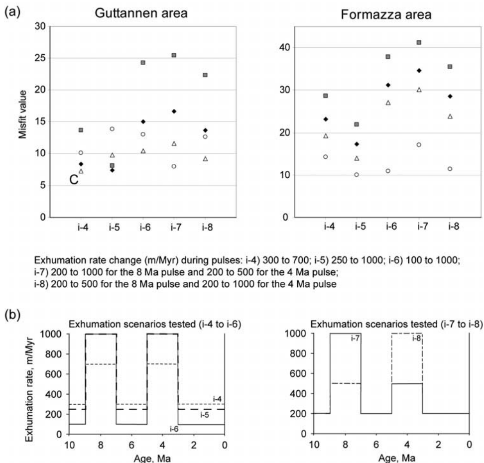
Figure 13. (a) Cumulated misfit between predicted and measured AFT and AHe ages in the Guttannen and the Formazza study areas for different intensities (i-4, i-5, i-6, i-7, i-8) of two 2-Ma-long exhumation pulses centered at 8 and 4 Ma and a choice of relief variation. Diamonds, steady relief; squares, relief reduction from \beta = 1.5 to 1; triangles, relief increase from \beta = 0.5 to 1; circles, temporary relief increase from \beta = 1 to 1.5 during exhumation pulses. See text for further details on the method. C ( \mu = 7.2 ) refers to case C in Figure 15. (b) Illustration of the five different exhumation rate scenarios tested, with i-4, i-5, i-6, i-7, or i-8 intensity variation centered at 8 or 4 Ma as detailed in the legend.
