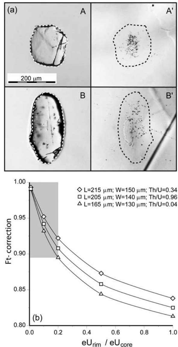
Figure 8. (a) Two examples of internal U zoning in apatites dated in this study, as recorded by the distribution of induced track in mica detectors used for AFT dating (A and A', sample AV4; B and B', sample AV2). The area covered by induced fission tracks in the mica detector (A', B') is clearly smaller than the polished area of the corresponding crystals (A, B). Dashed lines indicate the grain contour. In both cases, the outer U-poor layer is 30\text{--}40\ \mu\text{m} thick. (b) Predicted Ft correction factor from a Monte Carlo model of He ejection [Gautheron et al. , 2008] for different crystal sizes (length L, width W), Th/U ratios (provided in key) and U depletion in a 30\ \mu\text{m} wide rim ( eU_{\text{rim}}/eU_{\text{core}} , with eU the effective uranium concentration as in the work by Shuster et al. [2006]). Grain sizes, Th/U ratios, and rim widths are characteristic of samples in this study. Shaded box corresponds to inferred range of Ft corrections applicable to our samples (compare to "standard" Ft correction for unzoned apatite; eU_{\text{rim}}/eU_{\text{core}} = 1 ).
