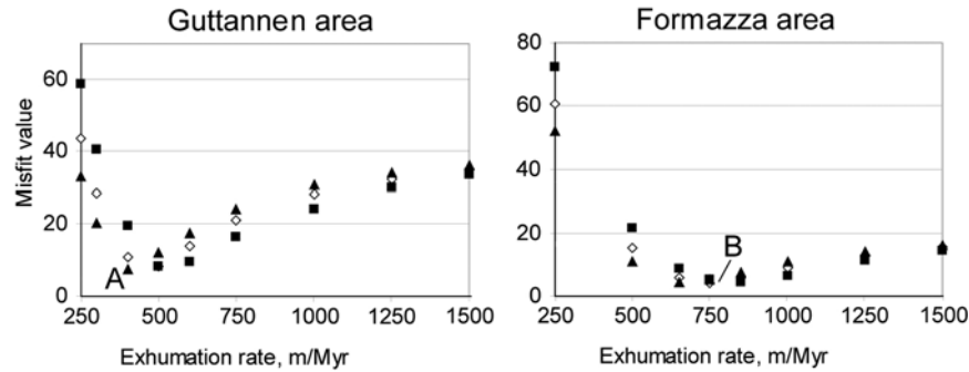
Figure 11. Cumulated misfit between predicted and measured AFT and AHe ages in the Guttannen and the Formazza study areas for different values of steady exhumation rate (plotted on x axis) and relief variation. Diamonds, steady relief; squares, relief reduction from \beta = 1.6 to 1; triangles, relief increase from \beta = 0.4 to 1. A ( \mu = 7.4 ) and B ( \mu = 4.4 ) refer to cases A and B in Figure 15. See text for details on the method.
