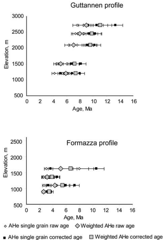
Figure 5. Spread of single-grain uncorrected (white diamonds) and corrected (black squares) AHe ages with 1\sigma analytical uncertainty, compared to weighted-average AHe ages (weighted according to 1\sigma analytical uncertainty; gray diamonds and squares, respectively, with error bars as explained in Table 3) for the Guttannen and Formazza elevation profiles.
