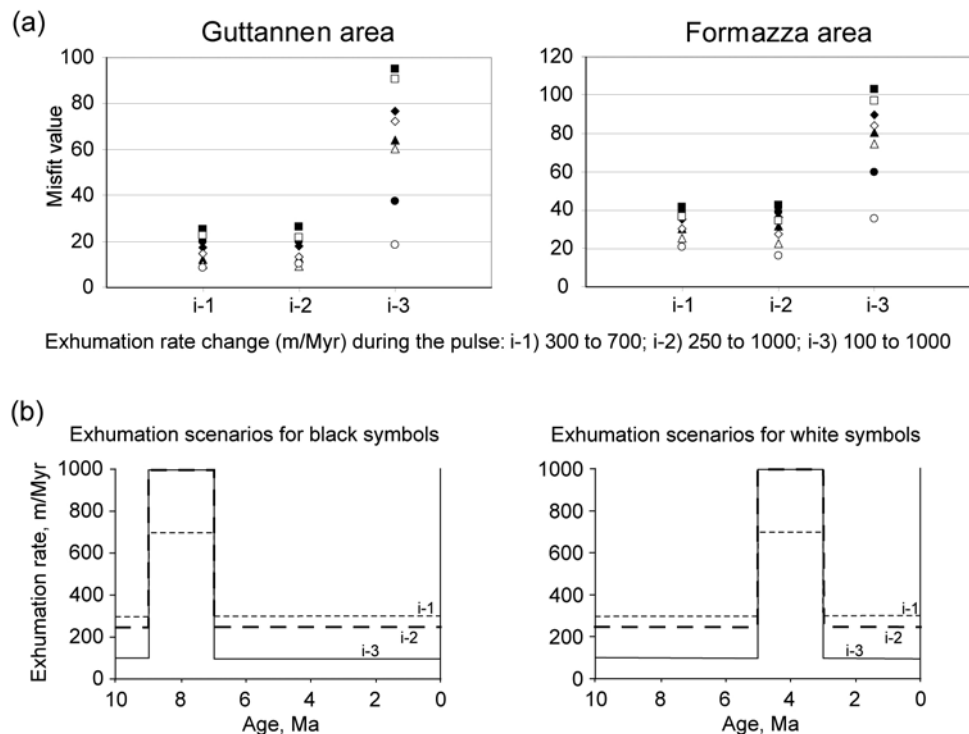
Figure 12. (a) Cumulated misfit between predicted and measured AFT and AHe ages in the Guttannen and the Formazza study areas, for different intensities (i-1, i-2, i-3) of 2-Ma-long exhumation pulses centered at either 8 Ma (black) or 4 Ma (white) and a choice of relief variation. Diamonds, steady relief; squares, relief reduction from \beta = 1.5 to 1; triangles, relief increase from \beta = 0.5 to 1; circles, temporary relief increase from \beta = 1 to 1.5 during exhumation pulses. See text for further details on the method. (b) Illustration of the 6 different exhumation rate scenarios tested, centered at 8 or 4 Ma and with i-1, i-2, or i-3 intensity variation as detailed in the legend.
