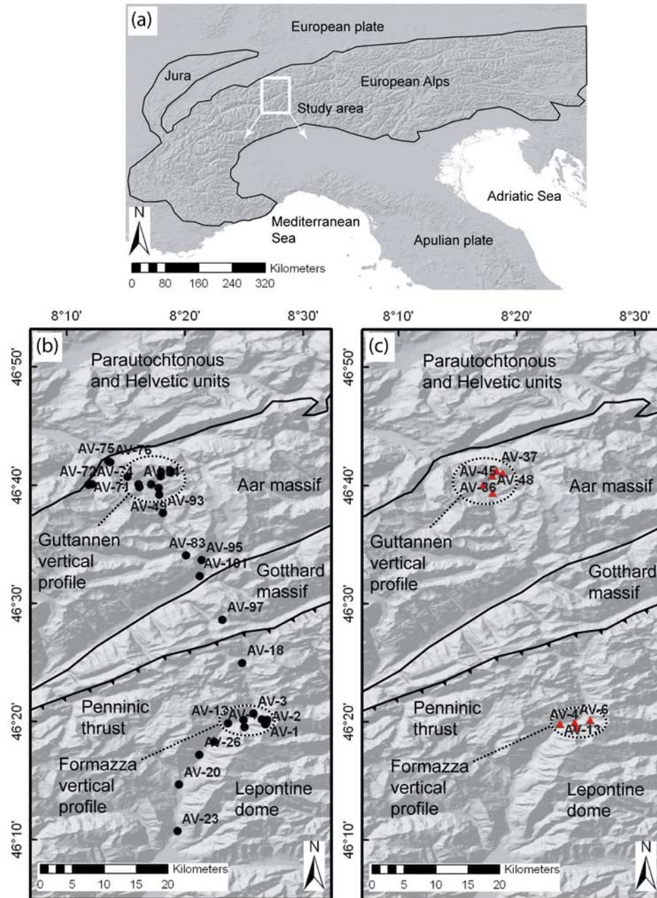
Figure 2. (a) Location map. Maps of (b) AFT and (c) AHe sampling, overlain on shaded relief model of study area (see Figure 2a for location). Main tectonic units and structures are also indicated.
