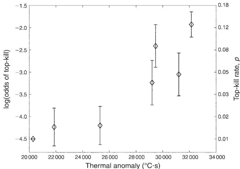
FIG. 2. Mortality rate of trees >5 cm dbh on each plot vs. mean thermal anomaly (°C·s). Probability, p , is transformed to the log odds (or logit, \ln(p/1 - p) ), where \ln is the natural logarithm) on the left axis, but is shown untransformed on the right. For a linear fit, r^2 = 0.82 ; P = 0.005 for log odds of top-kill vs. thermal anomaly. Zero mortality ( -\infty log odds) is shown as -4.5 and is fitted as such. Error bars show \pm SD, estimated by bootstrapping.
