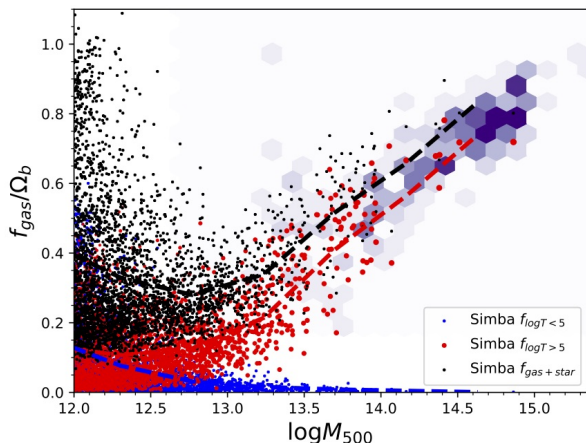
Figure 12. Gas fractions as a function of M_{500} at z = 0 . Black points show the total baryon fraction within the halo, and red and blue points show the gas fractions subdivided at 10^5\text{K} . Purple hexbins show an observational compilation of hot gas fractions from McCarthy et al. (2017), to be compared to the red points. SIMBA does a reasonable job of reproducing the observed trend of hot gas fraction with M_{500} , which has been difficult for previous simulations to achieve without tuning.
