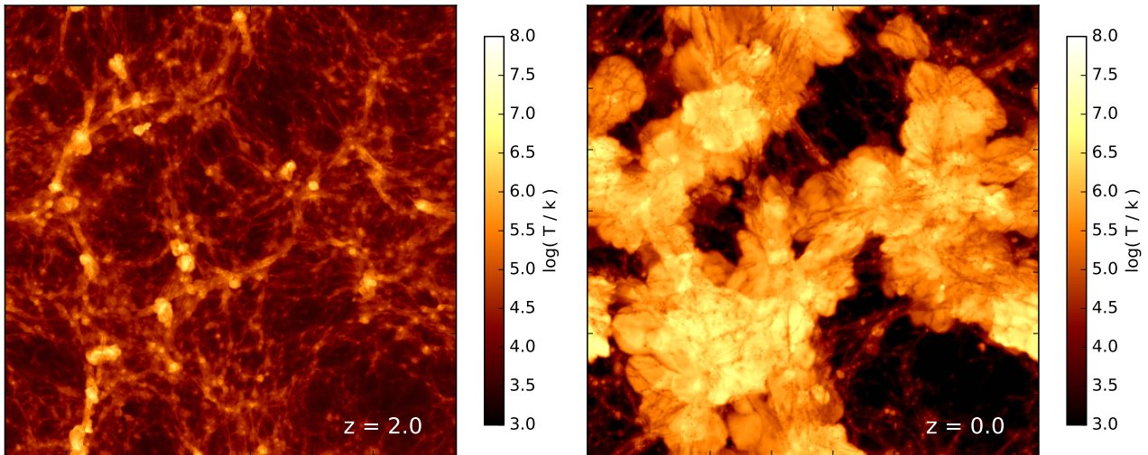
Figure 2. Temperature map projected through a random 10 Mpc/h slice from a 50 Mpc/h SIMBA volume, at z = 2 (left) and z = 0 (right). At z = 2 , warm-hot gas traces large-scale filaments, with energetic bipolar outflows owing to jets evident from the nodes where the most massive galaxies and black holes reside. At z = 0 , high-speed AGN outflows have shocked the IGM gas throughout much of this volume to well beyond the virial radii of halos, with cooler dense filamentary structures penetrating the hot gas.
