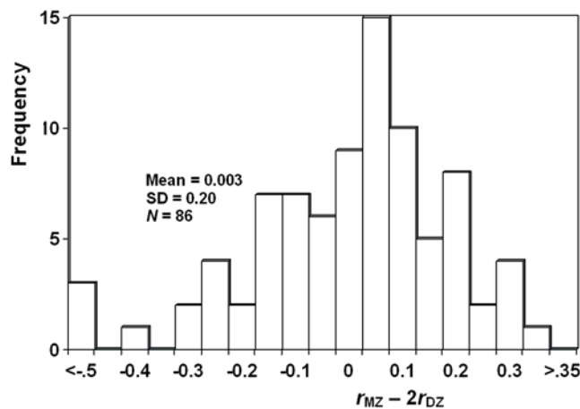
Figure 1. Distribution of r_{MZ} - 2r_{DZ} for all traits on human twins. Data are from published papers by N.G. Martin and colleagues of the Queensland Institute of Medical Research, Brisbane ( www.genepi.edu.au ). Across a wide variety of traits the mean difference between the monozygotic twin correlation and twice the dizygotic twin correlation is close to zero, which is consistent with predominantly additive genetic variance and the absence of a large component of variance due to common environmental effects. doi:10.1371/journal.pgen.1000008.g001
