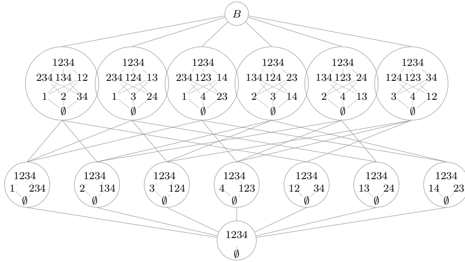
FIGURE 4. The poset of subalgebras of a 16-element Boolean algebra
