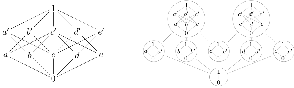
FIGURE 1. The orthoalgebra on the left is constructed from gluing together two Boolean algebras \{0, a, b, c, a', b', c', 1\} and \{0, c, d, e, c', d', e', 1\} . The orthogonal sum \oplus is the union of the orthogonal join operations of these Boolean algebras. On the right is the Hasse diagram of its poset of Boolean subalgebras.
