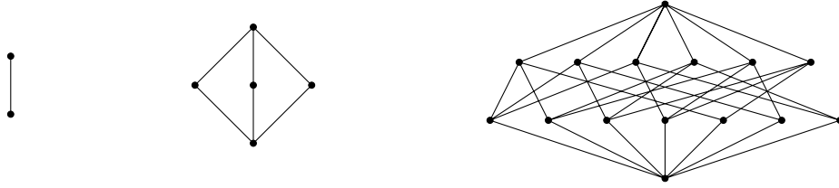
FIGURE 2. Hasse diagrams of the posets \text{BSub}(A) for Boolean algebras A with 4, 8, and 16 elements. A Boolean algebra with 4 elements has two subalgebras: \{0, 1\} , and itself. A Boolean algebra A with 8 elements has five subalgebras: \{0, 1\} , three subalgebras \{0, a, a', 1\} for a \in A \setminus \{0, 1\} , and A itself. A Boolean algebra with 16 elements has a more complicated structure of subalgebras, containing subalgebras with 2, 4, 8, and 16 elements.
