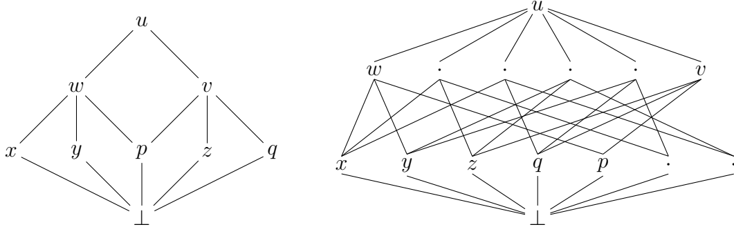
FIGURE 6. A part of the Hasse diagram of the shadow from the proof of Lemma 5.6 (two possible partial diagrams of the same situation)
