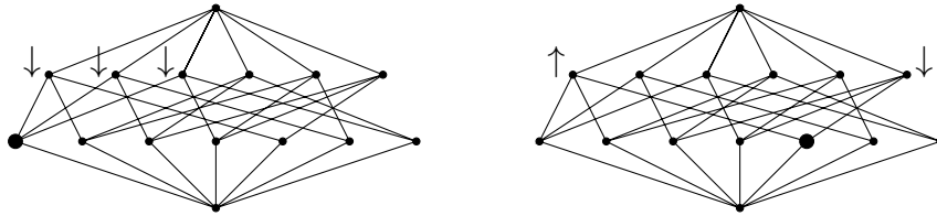
FIGURE 5. Direction for a distinguished atom in a 16-element Boolean algebra
