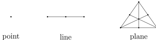
FIGURE 3. Hypergraphs of the examples from Figure 2.
