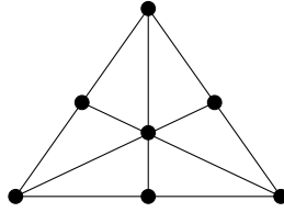
FIGURE 7. The hypergraph view of the subalgebras of a 16-element Boolean algebra
