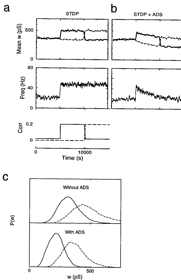
Figure 5. Competition between synaptic inputs and the effect of activity-dependent scaling (ADS). a , Behavior of model without ADS. Bottom graph , The neuron receives input from two sets of 50 synapses. Until time 5000 sec, both sets are uncorrelated. At 5000 sec the inputs within one set become strongly correlated, potentiating its weights. At 10,000 sec this set becomes again uncorrelated, whereas the other set becomes correlated, reversing the situation. Middle graph , The postsynaptic firing frequency jumps when the inputs become correlated. Top graph , The average synaptic weight for the two sets. The introduction of correlation potentiates the synapses, but changes in one group of synapses barely affect the other group. Competition is almost absent. b , Same situation but with activity-dependent scaling turned on. After the jump in firing rate the synapses are slowly scaled downward, until the activity is again at its goal value of 20 Hz. This introduces competition. Note the difference in time-scales between the slow competition and the much faster STDP. c , The corresponding weight distributions once equilibrium has been reached. The activity-dependent scaling scales the weights of both groups.
