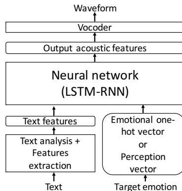
Figure 1: Flowchart for the proposed RNN speech synthesis system using emotional one-hot or perception vectors.
