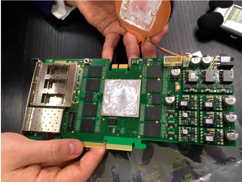
Figure 4 A field-programmable gate array (FPGA) in a 'development kit' for programming and testing. The FPGA is the large central chip with white paste on it. Source: Author's fieldwork photograph.
