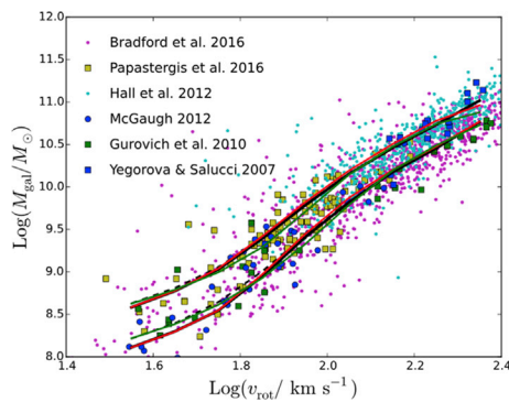
Fig. 3. BTF relation reproduced by GalICS2.0, where data points in different colors correspond to observed galaxies with data from McGaugh, 2012, Gurovich, Freeman, Jerjen, Staveley-Smith, and Puerari (2010) and so on. The color-coded curves correspond to the default model for GalICS2.0 in black solid, and three variations of it (labelled 'model 1, 2, and 3') in red, black dashed and green. © Cattaneo et al. (2017), p. 1420.
