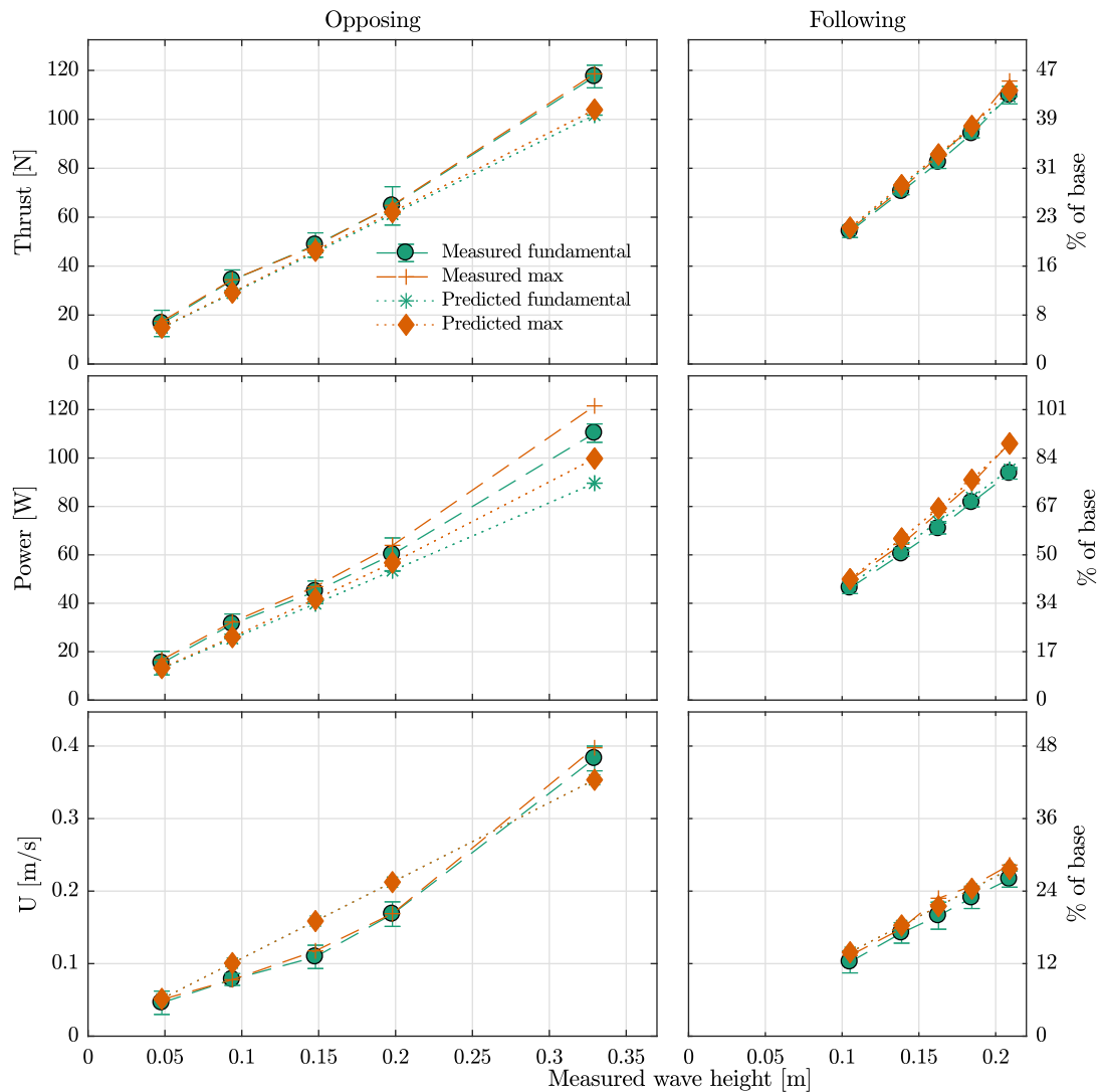
Fig. 12. Wave induced fluctuations in various parameters as a function of wave amplitude. Shown for opposing and following waves at 0.4 Hz in a mean current velocity of 0.81 m/s, along with predicted values. Error bars denote the standard deviation between the 5 repeats. Left hand axis shows absolute wave-induced fluctuations, whilst right hand axis shows these variations as a percentage of current only values.
