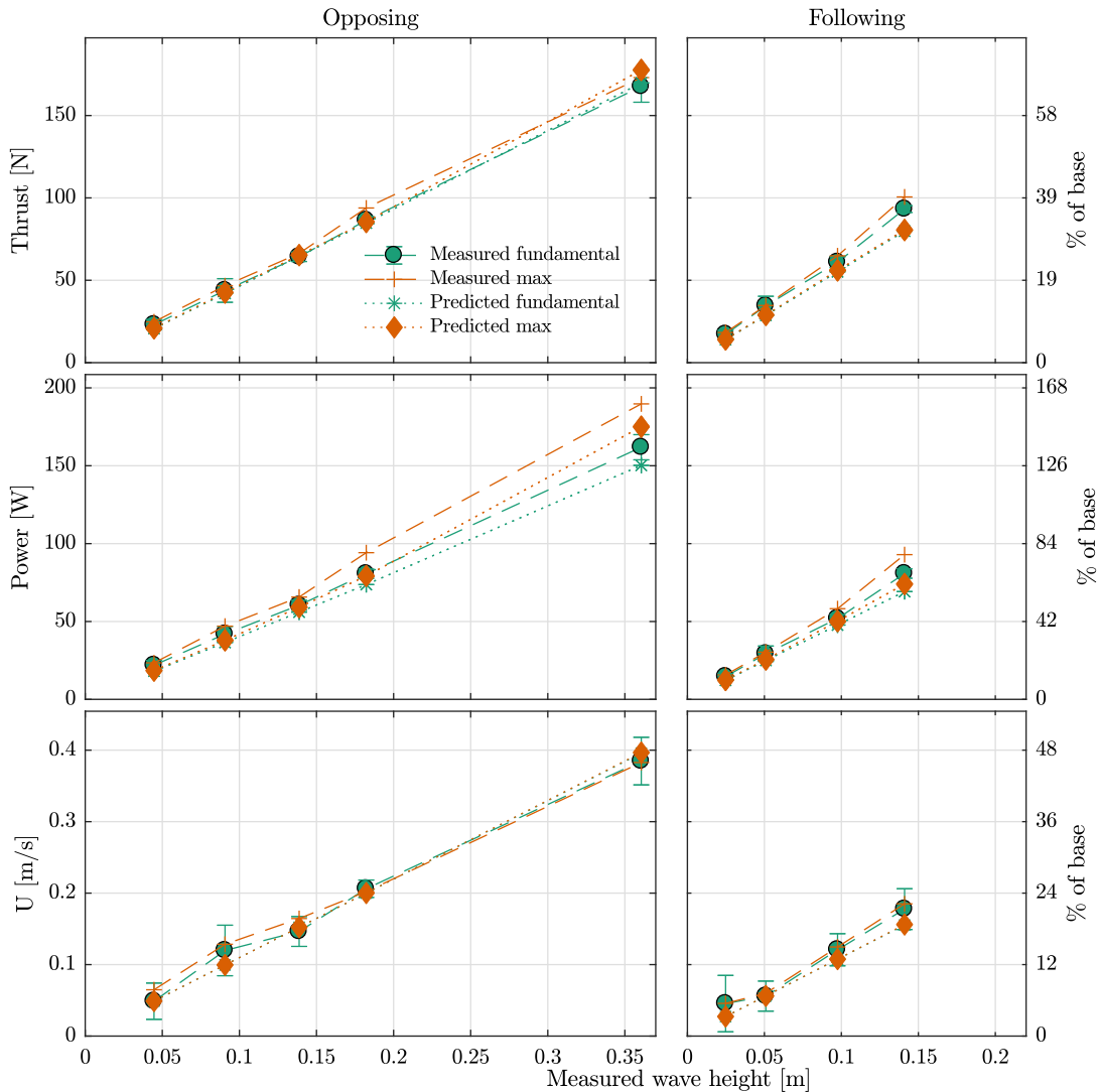
Fig. 11. Wave induced fluctuations in various parameters as a function of wave amplitude. Shown for opposing and following waves at 0.31 Hz in a mean current velocity of 0.81 m/s, along with predicted values. Error bars denote the standard deviation between the 5 repeats. Left hand axis shows absolute wave-induced fluctuations, whilst right hand axis shows these variations as a percentage of current only values.
