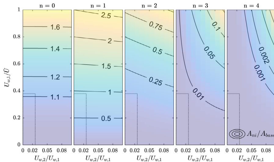
Fig. 8. Contours of theoretical Fourier coefficients in the thrust spectrum relative to the mean thrust without waves. Shown for various wave velocities relative to the mean flow, and various degrees of wave non-linearity. The region enclosed by dotted lines indicates that explored in the presented experimental test programme.
