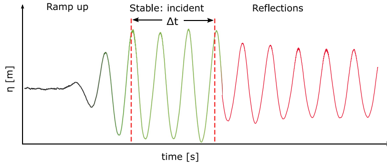
Fig. 6. Example of a stable region of waves used for snippet analysis. Ramp up, stable and regions with reflections shown.
