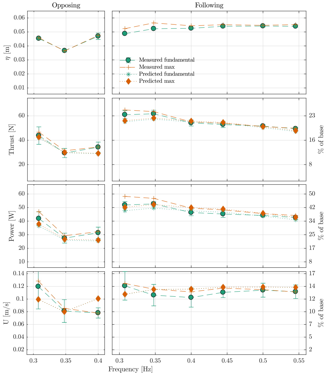
Fig. 14. Wave induced fluctuations in various parameters as a function of wave frequency. Shown for opposing and following waves in a mean current velocity of 0.81 m/s. Error bars denote the standard deviation between the 5 repeats. Left hand axis shows absolute wave-induced fluctuations, whilst right hand axis shows these variations as a percentage of current only values.
