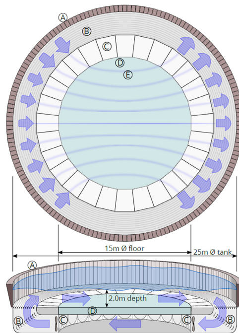
Fig. 3. Schematic of FloWave in plan and oblique section (from Sutherland et al., 2017) showing: (A) Wavemaker paddles around circumference (168 Nr); (B) Turning vanes and flow conditioning filters; (C) Current drive impeller units (28 Nr); (D) Buoyant raisable floor (15 m \varnothing ) below test area; (E) Idealised streamlines of flow across tank floor.
