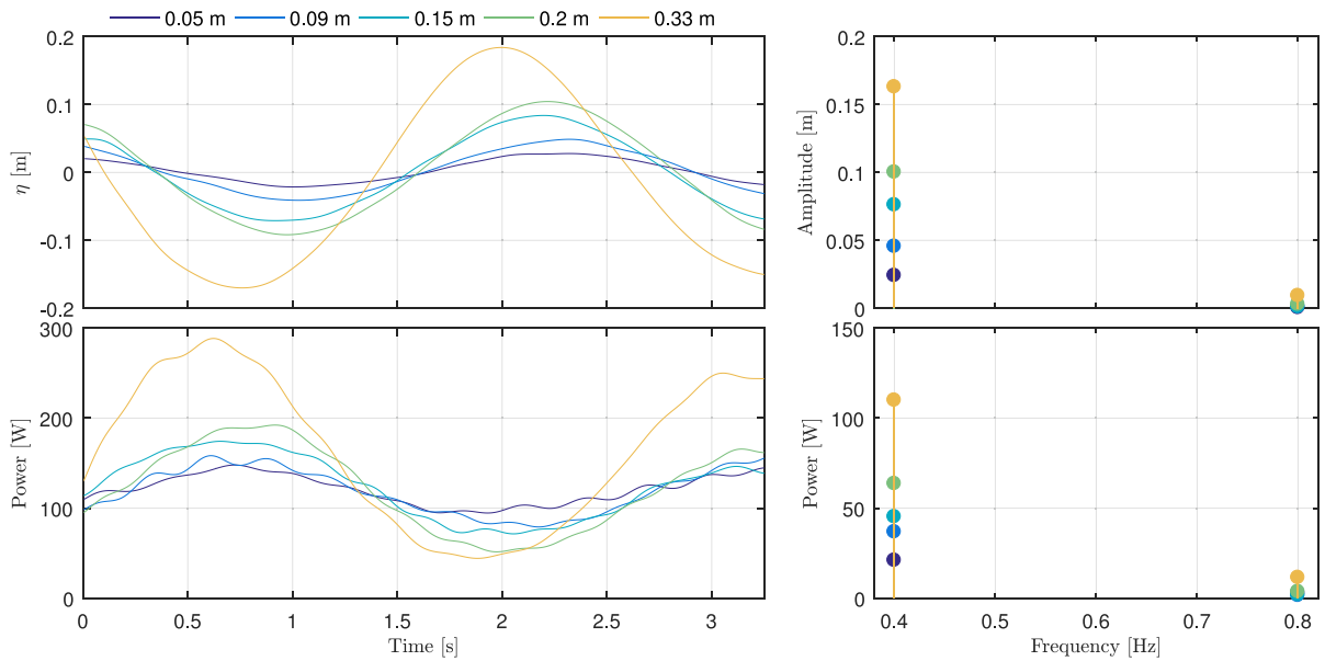
Fig. 10. Frequency and time-domain examples of surface elevation and corresponding variations in power. One repeat of each of the 5 amplitudes at 0.4 Hz shown in opposing current. Time-series data is low pass filtered at 4 Hz to aid visibility.
