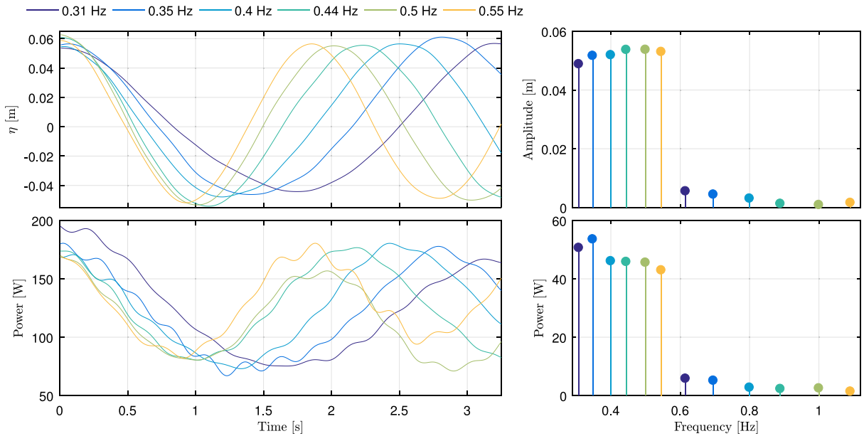
Fig. 13. Frequency and time-domain examples of surface elevation and corresponding variations in power. Shown for 6 frequencies with a single target amplitude, in following current. Time-series data is low pass filtered at 4 Hz to aid visibility.
