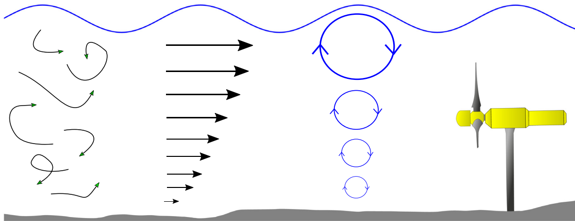
Fig. 1. Diagram of the causes of unsteady loads on tidal turbines. Shown from left to right: turbulence, shear flow and waves.
