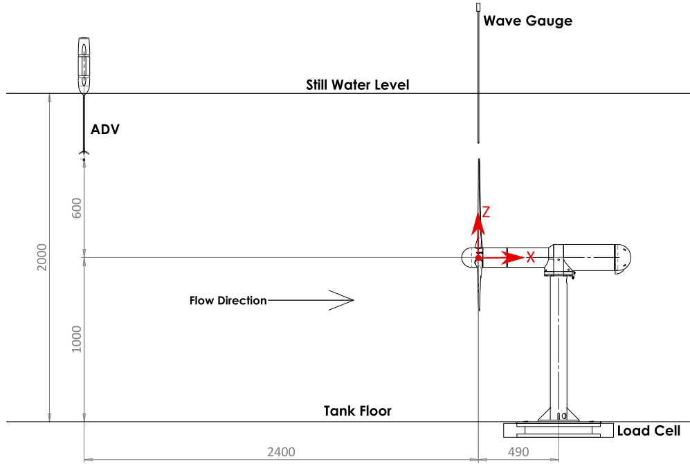
Fig. 4. Location of test instrumentation in the FloWave basin relative to the rotor plane (dimensions in mm).
