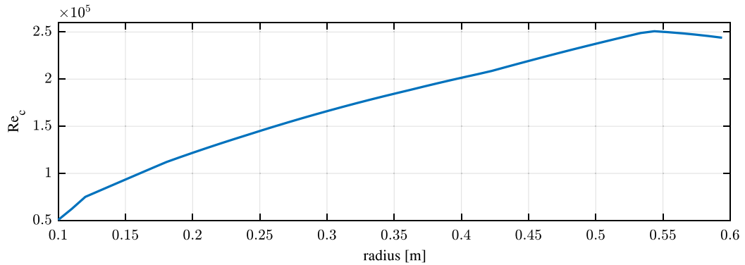
Fig. 5. Chord based Reynolds number variation with local radius.
