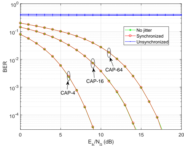
Fig. 11. Comparison of BER performance of CAP with no jitter, with and without synchronization for different constellation sizes in VLC system, \tau = 0.25T and P = 11 .
