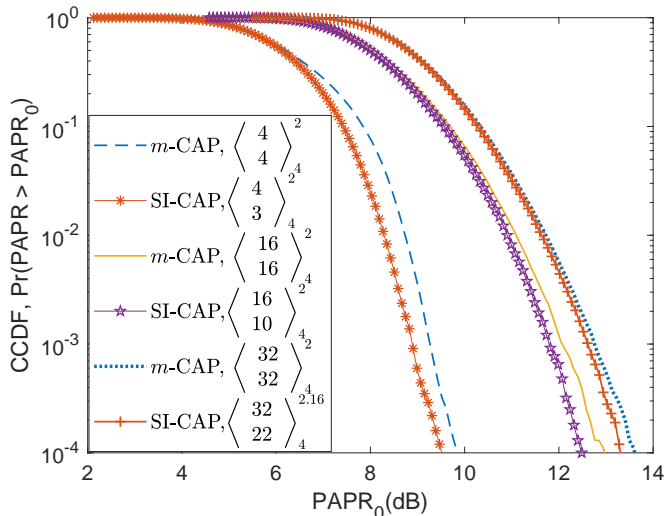
Fig. 22. The comparison of complimentary cumulative density function (CCDF) of the peak to average power ratio (PAPR) of SI-CAP and m -CAP for varying number of subbands.
