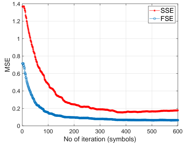
Fig. 17. MSE convergence rate of FSE and SSE for CAP-16 at R_b = 30 Mb/s and SNR=20 dB.
