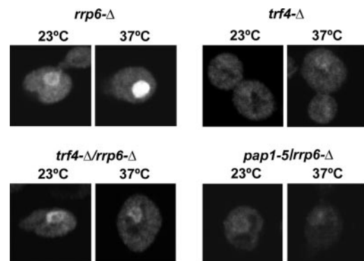
FIG. 8. Trf4 and Pap1 are required for formation of the poly(A) domain in the rrp6Δ mutant. All strains were grown at 23°C in YPD medium to early/mid-log phase. Poly(A) + RNA was detected by FISH in cells that were either grown at 23°C or incubated for 1 h at 37°C, as indicated.
