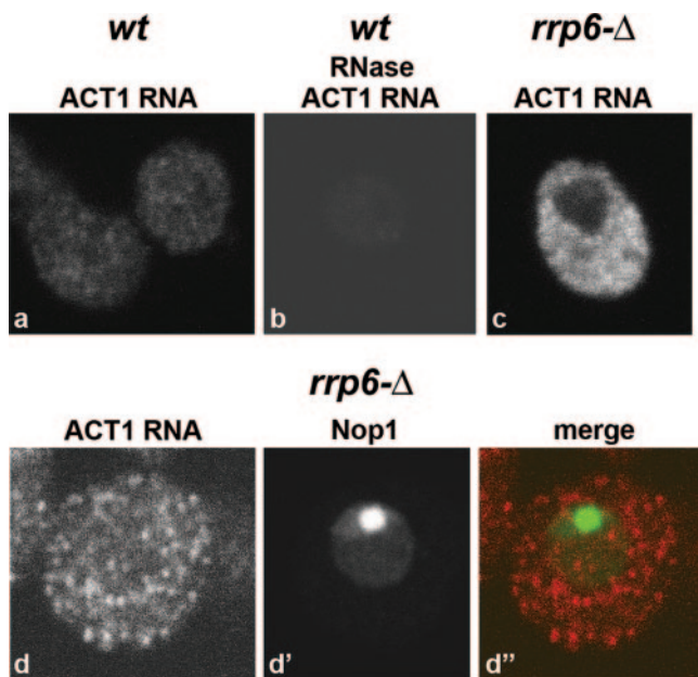
FIG. 4. Localization of actin mRNA ( ACT1 RNA ) in wild-type and rrp6 \Delta yeast strains. Cells were grown at 23°C and incubated for 1 h at 37°C. FISH was performed using oligonucleotide probes complementary to the coding sequence of actin mRNA. For a direct comparison of staining intensities, images were acquired with the same confocal settings. wt, wild type.
