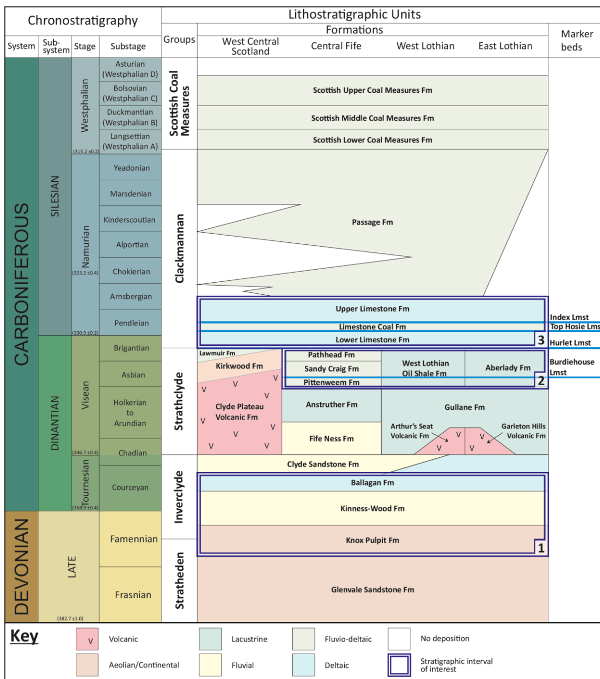
Figure 3: Lithostratigraphic nomenclature and stratigraphic succession. Also shown is the level of the three selected storage plays (blue boxes) discussed in the text from oldest to youngest. Modified from 41-44 .
