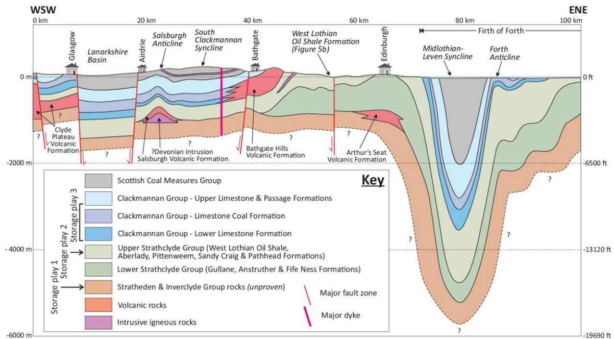
Figure 5: Simplified cross section through the Midland Valley showing some of the Groups and Formations that constitute the Palaeozoic fill of the basin. Adapted from Managhan 43 .
