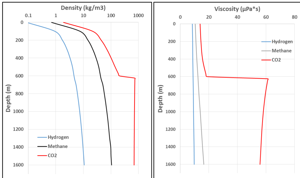
Figure 2: Density and viscosity changes of methane, CO 2 and hydrogen with depth calculated using the NIST database 29 . The geothermal gradient is based on data mainly taken from the Midland Valley region 30 and a pressure gradient based on a freshwater pore fluid density of 1g/cm 3 .
