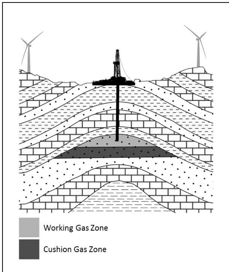
Figure 1: Simplified hydrogen storage scenario in a brine filled reservoir formation (dotted pattern) underneath an impermeable shale-rich sealing formation (dashed pattern). For simplicity, the injection well also acts as the production well. The anticlinal shape of the structure prevents the hydrogen from migrating away from the well. The reproducible gas ('working gas') as well as the cushion gas volume are highlighted.
