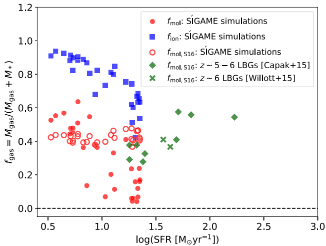
Figure 13. Molecular gas mass fractions of our simulations and of the z \sim 5\text{--}6 LBGs observed by Capak et al. (2015) and Willott et al. (2015). The filled and open red circles indicate true fractions inferred directly from the simulations and fractions inferred from the parametrizations in Scoville et al. (2016), respectively. Applying this parametrization to the z \sim 5\text{--}6 LBGs gives the molecular gas mass fractions shown by the green diamonds and crosses. Also shown are the true ionized gas mass fraction of our simulations (blue filled squares).
