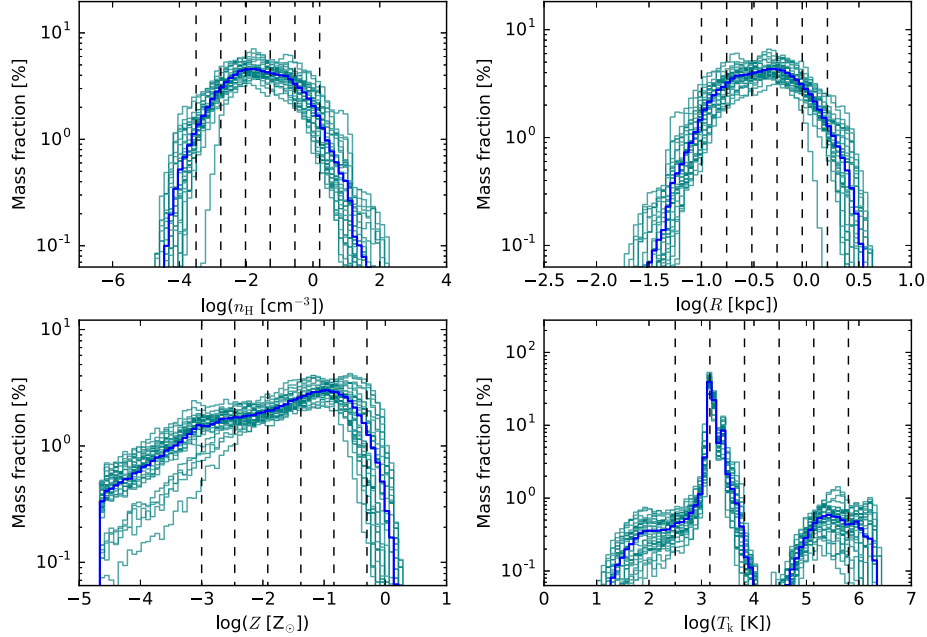
Figure 5. Histograms of n_{\text{H}} , R , Z , and T_{\text{k}} of the diffuse gas clouds in our 30 model galaxies (dark green histograms), with the mean histograms shown in blue. The vertical dashed lines indicate the chosen CLOUDY grid points (see Section 3.3).
