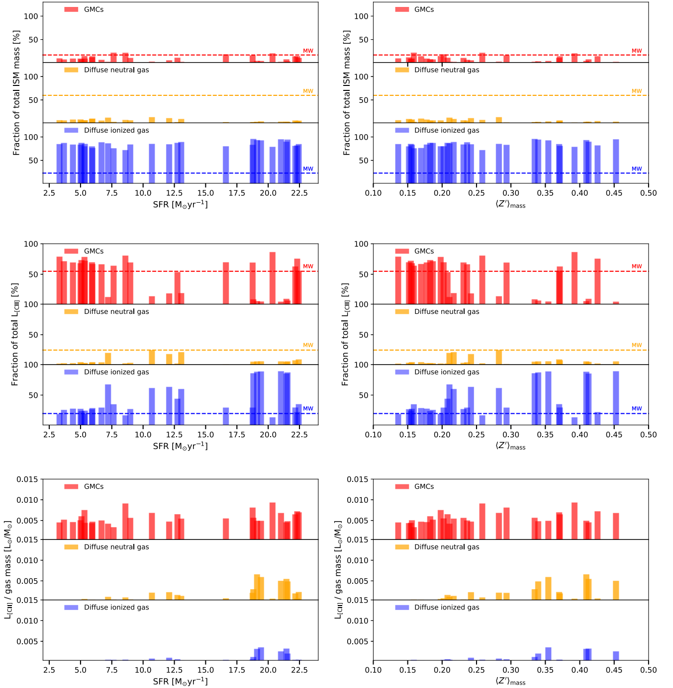
Figure 7. Top: mass fractions of the three ISM phases of our simulated galaxies as a function of their total SFRs (left panel) and mass-weighted average metallicities, \langle Z \rangle_{\text{mass}} (right panel). The three ISM phases, GMCs, diffuse neutral gas, and diffuse ionized gas, are shown as red, orange, and blue shaded regions, respectively. The corresponding mass fractions in the MW have been shown with horizontal dashed lines: 17% \text{H}_2 (red), 60% \text{H I} (orange), and 23% \text{H II} (blue) within 20 kpc with numbers from Draine (2011). Middle: the contributions from the ISM phases to the total [\text{C II}] luminosities vs. SFRs (left panel) and \langle Z \rangle_{\text{mass}} (right panel). The horizontal dashed lines indicate the corresponding fractions for the MW (Pineda et al. 2014). Bottom: the [\text{C II}] luminosity per gas mass of each ISM phase vs. SFRs (left panel) and \langle Z \rangle_{\text{mass}} (right panel).
