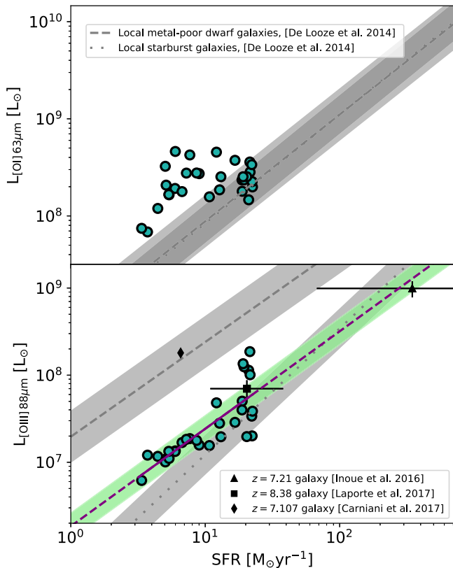
Figure 8. L_{[O I]} vs. SFR (top) and L_{[O III]} vs. SFR (bottom) for our simulated galaxies (filled circles) compared to the z \gtrsim 5 observations of the two lines. A log-linear fit to the [O III] simulations is shown by the purple dashed line with a 1\sigma scatter (0.15 dex) in L_{[O III]} as indicated by the green shaded region. Local relations for metal-poor dwarf galaxies (gray dashed lines) and local starburst galaxies (gray dotted lines) are shown for comparison (De Looze et al. 2014). The gray shaded regions indicate the \pm 1\sigma scatter around these relations. Also shown are the detections to date of [O III] in star-forming galaxies at z \gtrsim 5 (Inoue et al. 2016; Carniani et al. 2017; Laporte et al. 2017).
