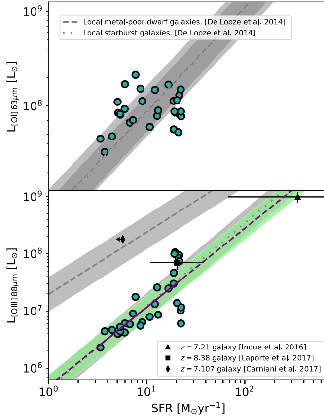
Figure 8. L_{[O I]} vs. SFR (top) and L_{[O III]} vs. SFR (bottom) for our simulated galaxies (filled circles) compared to z \gtrsim 5 observations of the two lines. A log-linear fit to the [O III] simulations is shown by the purple dashed line with a 1\sigma scatter (0.15 dex) in L_{[O III]} as indicated by the green shaded region. Local relations for metal-poor dwarf galaxies (gray dashed lines) and local starburst galaxies (gray dotted lines) are shown for comparison (De Looze et al. 2014). The gray-shaded regions indicate the \pm 1\sigma scatter around these relations. Also shown are the detections to date of [O III] in star-forming galaxies at z \gtrsim 5 (Inoue et al. 2016; Carniani et al. 2017; Laporte et al. 2017).
