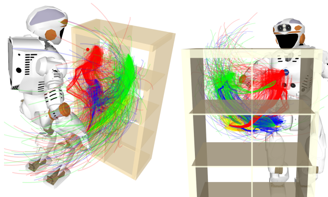
Fig. 1: Pick-and-place scenario in a complex environment with collision avoidance. A humanoid robot has to retrieve an item from a shelf, the target of which may change based on perception information or user input. In order to synthesize optimal motion fast online, we investigate different warm-start strategies for trajectory optimization methods.
