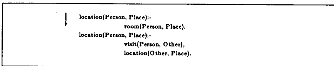
Figure 9: Order of Attempted Unification
