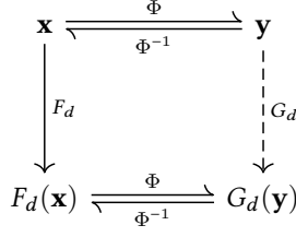
Fig. 1. Commutative diagram between F_d and G_d .
