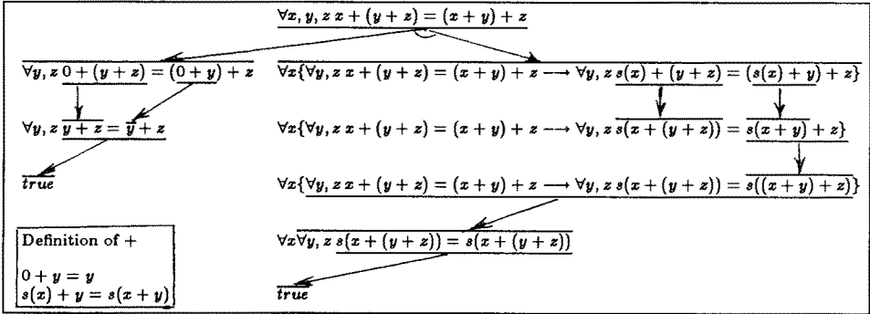
Figure 1: Proof of the Associativity of +
