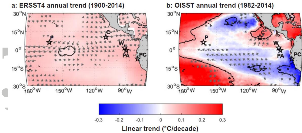
Figure 4. Linear trends in in tropical year-averaged ETP SST gridded datasets (colors). Contours indicate significance at p < 0.05 (in (a), significant area is outside contoured shape). Vectors show significant linear trends ( p < 0.05 ) in 20CR v2 winds at 1000 mbar; longest vector (in (a)) is 3.8 m/s.
