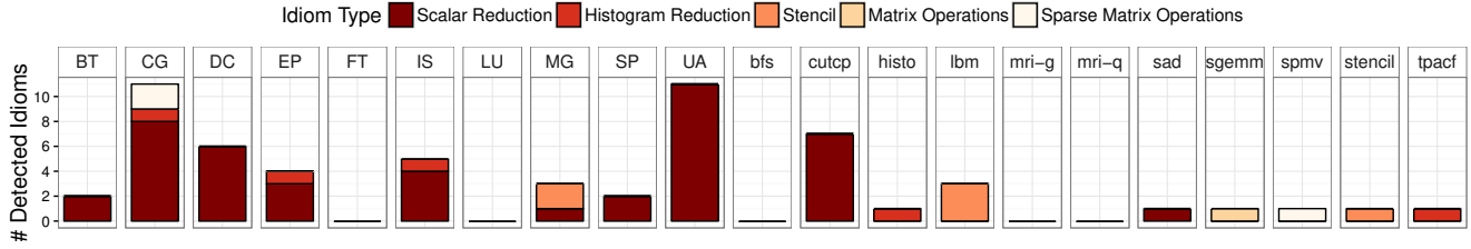
Figure 16. The different computational idioms found in all benchmarks.
