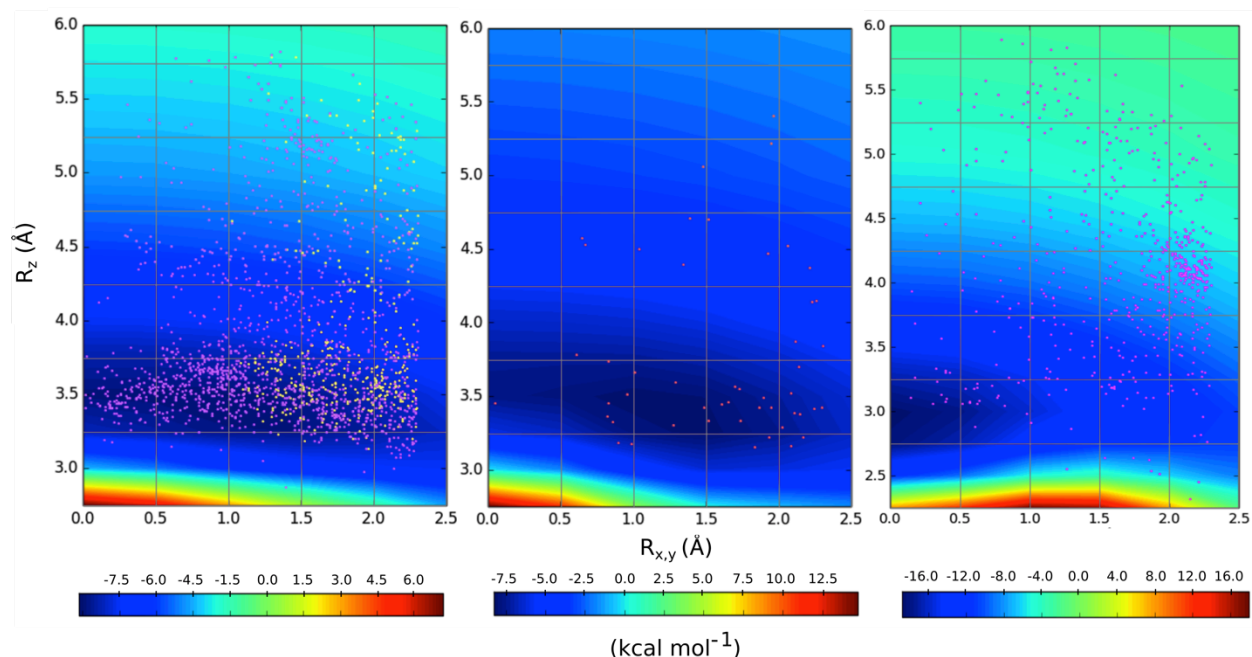
Figure 6. Empirical distribution of complexes (points) superimposed on the computed DLPNO-CCSD(T)/aug-cc-pVTZ potential energy surface (in kcal mol -1 ); (left) Arg-aromatic primary (purple) and secondary bicyclic (yellow), (middle) His-aromatic, and (right) Lys-aromatic complexes.
