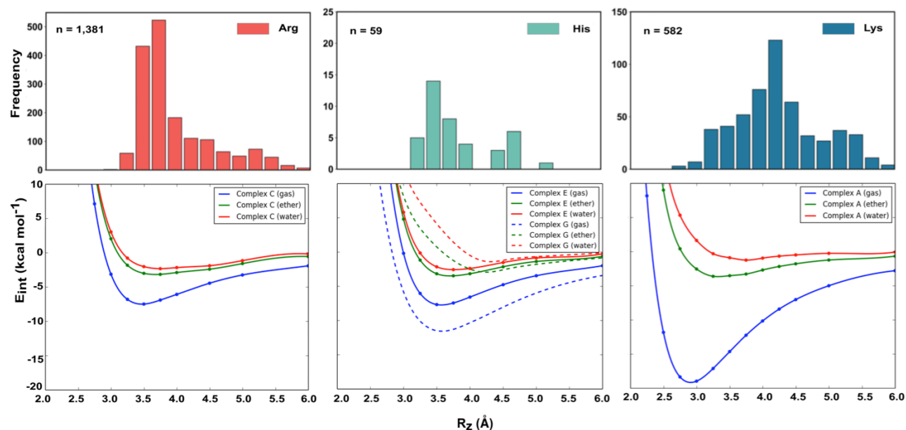
Figure 7. Normalized distance dependence of empirical interactions (bars) compared against DLPNO-CCSD(T)/aug-cc-pVTZ computed potential energy curves ( \text{kcal mol}^{-1} ) in the gas phase and with a dielectric constant of 4.2 (diethyl ether) and 78.4 (water). Solvation corrections were computed at the CPCM-MP2/cc-pVTZ level of theory.
