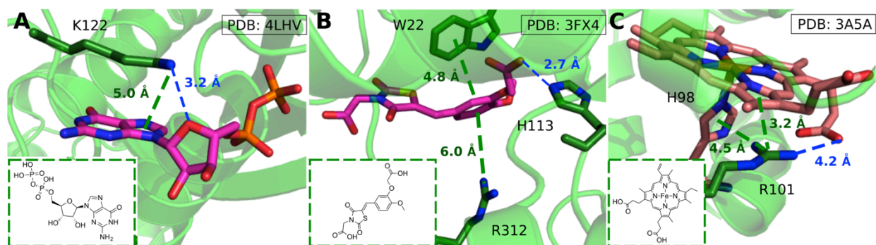
Figure 8. (A) GDP/GTP Lys-aromatic binding site selected from ammonium-PES R_{x,y} , R_z , \approx (2.0, 4.0) (ligand ID GDP). Examples of Arg-aromatic cation- \pi (B) long distance (ligand ID FX4) and (C) short distance bond (ligand ID HEM).
