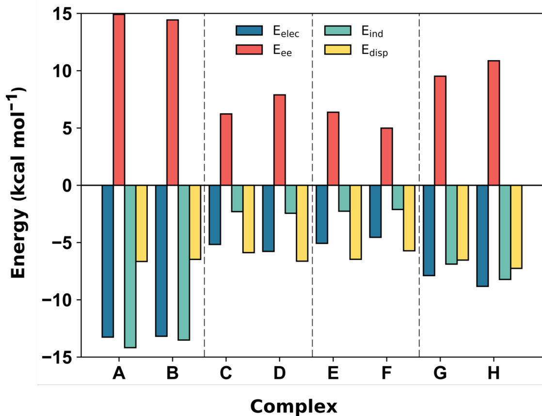
Figure 5: SAPT2+3/aug-cc-pVDZ decomposition of the interaction energy (in kcal mol -1 ) into exchange repulsion ( E_{ee} , red), electrostatics ( E_{elec} , blue), induction-polarization ( E_{ind} , green) and London dispersion ( E_{disp} , yellow) at the equilibrium separation.
