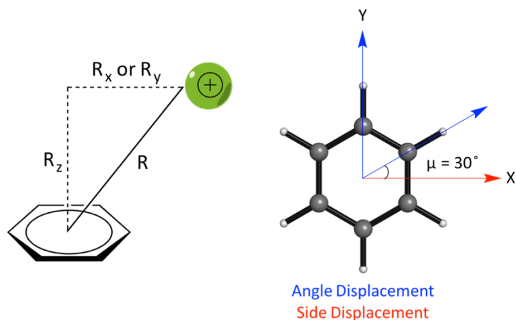
Figure 3. (Left) Parameters describing the relative geometry for PEC calculations between the cation and benzene using the distance ( R ), vertical offset ( R_z , along the normal) and horizontal offsets ( R_x and R_y , parallel to the plane of benzene). (Right) The side and angle displacements of the cation relative to benzene corresponding to vectors pointing to a C–C/C–H bond by adjusting X and Y coordinates, used to describe the difference in geometry between pairs of complexes, e.g. (E) and (F).
