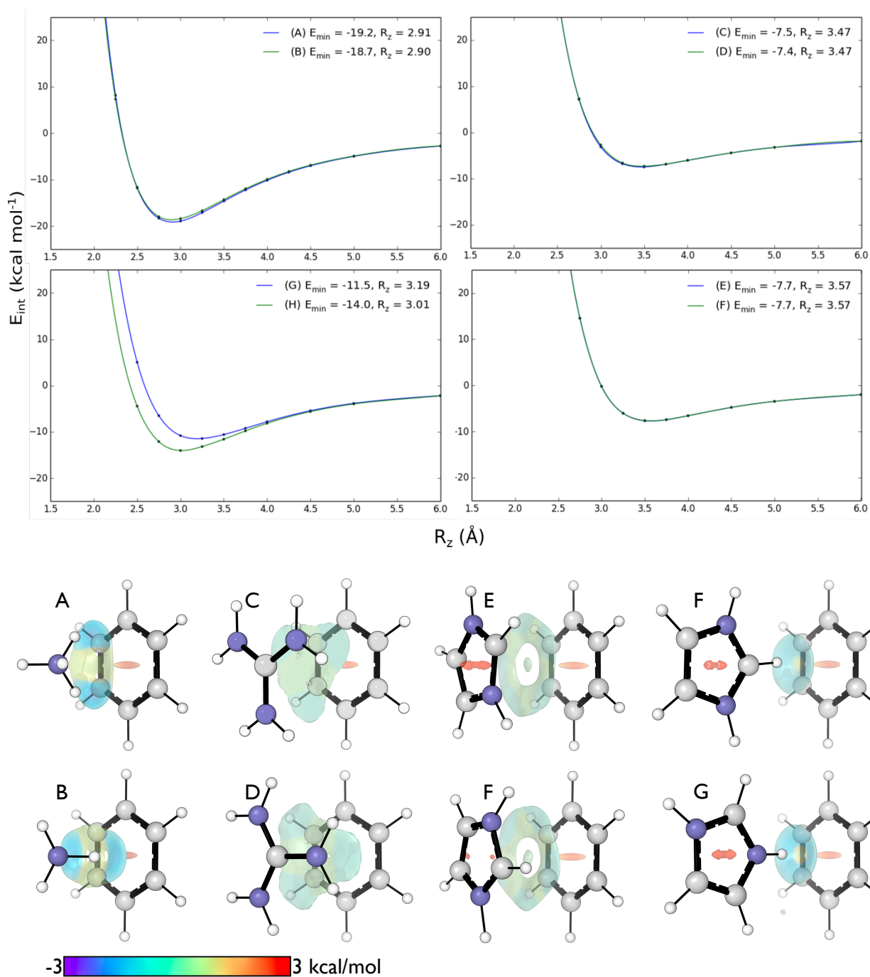
Figure 4. Top: DLPNO-CCSD(T)/aug-cc-pVTZ interaction energies (kcal mol -1 ) as a function of intermolecular separation of cation- \pi complexes. Minimum energies ( E_{\text{min}} ) and equilibrium separations ( R_z ) shown. Bottom: NCI isosurfaces at the minimum energy separations.
