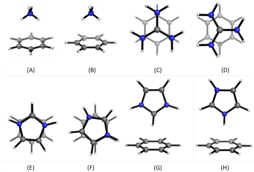
Figure 2. Cation- \pi complexes analyzed in this work. Models of (A)/(B) lysine; (C)/(D), arginine; and (E)-(H), histidine sidechains interacting with benzene.
