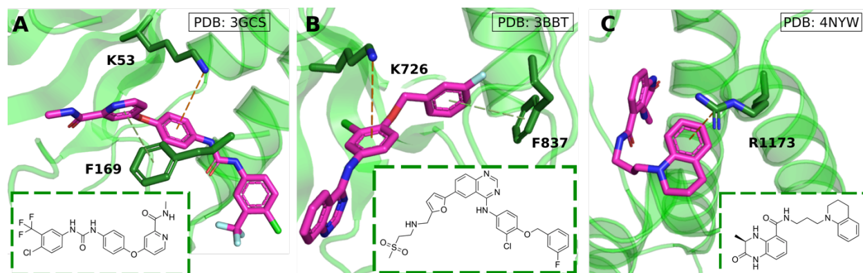
Figure 1. Aromatic ligands forming cation- \pi interactions with the target protein: A) Sorafenib complexed with Human p38 MAP kinase, B) Lapatinib in complex with ErbB4 kinase, C) Conway and co-workers' dihydroquinoxalinone inhibitor of the CREBBP bromodomain.
