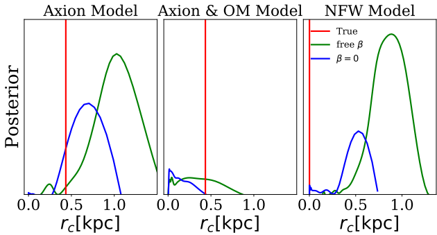
Figure 6. Same as Fig. ?? but for the core radius, r_c \approx r_{sol}/3 . The analysis with the constant anisotropy, \beta , set as free parameter tends to recover a larger core for the isotropic mocks (left and right panels). The analysis recovers a core radius closer to its true value when the analysis is done with \beta = 0 , but still with a significant bias. In the case of the axion with an Osipkov-Meritt anisotropy profile (middle panel), the analysis either with \beta = 0 or free \beta = \text{const.} , leads to very spread posterior distributions. In the case of anisotropic Osipkov-Meritt mock it is interesting to notice how the bias is towards smaller core radii, instead of large core radii, as opposed to the bias in the isotropic mocks.
