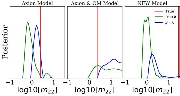
Figure 5. Posterior distribution for the axion mass from the Jeans analysis in the Fornax mocks for the axion with isotropic velocity dispersion (left), the axion with an Osipkov-Meritt anisotropy velocity dispersion profile (middle), and NFW density model with isotropic velocity dispersion (right). For isotropic axion (left) and NFW (right) mocks, the analysis with the anisotropy, \beta , set as free parameter tends to recover smaller axion mass (note that the NFW profile is similar to an axion one with large axion mass, Eq. (6), so that the core radius goes to zero). For the isotropic axion (left), only when the analysis is done with the true anisotropy, \beta = 0 , is that we recover an axion mass close to its true value, but still with a significant bias. For the anisotropic axion (middle) we recover a widely spread posterior, even though the maximum of the posterior coincides with the true value. Finally, the NFW isotropic (right) recovers a false core either with the isotropic or the constant anisotropic model.
