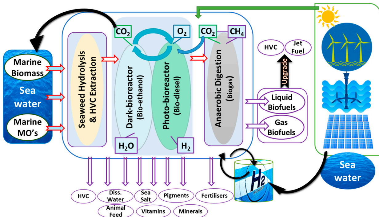
Figure 2. Coastal Integrated Marine Biorefinery (CIMB) system. Marine components (seawater, marine biomass, and marine microorganisms) serve as inputs for the biorefineries. Different biological and biochemical conversion processes are performed (blue box). Biofuels and high-value chemicals are obtained (purple arrows and ovals). Renewable energy sources (green box/arrow) are integrated with the biological system to improve efficiency.
