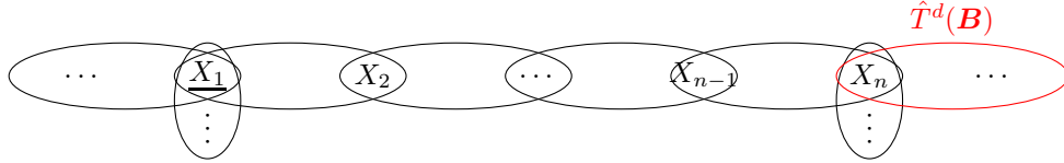
Figure 10: Illustration of a path in a query that does not have safe atom-to-variable paths.
