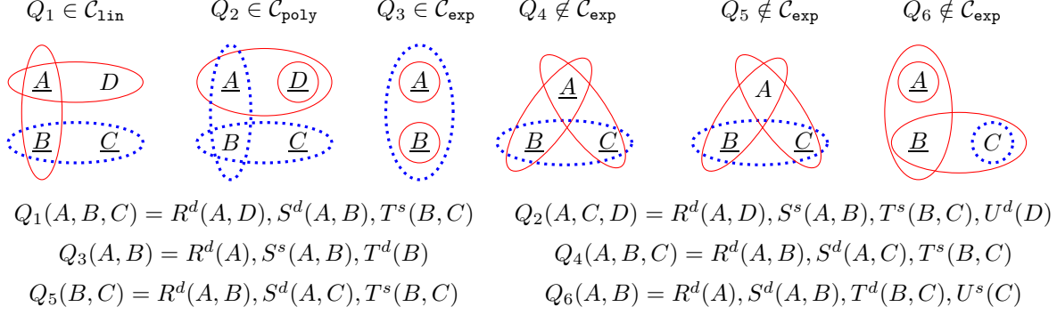
Figure 2: Examples of queries inside and outside our tractability classes. The static and dynamic relations are adorned with the superscripts s and respectively d . In the hypergraphs, there is one node per variable and one hyperedge per relation. Underlined variables are free. Solid (red) hyperedges denote the dynamic relations, the dotted (blue) hyperedges denote the static relations.
