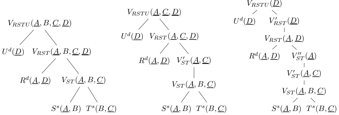
Figure 3: Three rewritings of the query Q_2(A, C, D) = R^d(A, D), S^s(A, B), T^s(B, C), U^d(D) from Figure 2. The first two rewritings are not safe, while the last one is safe.
