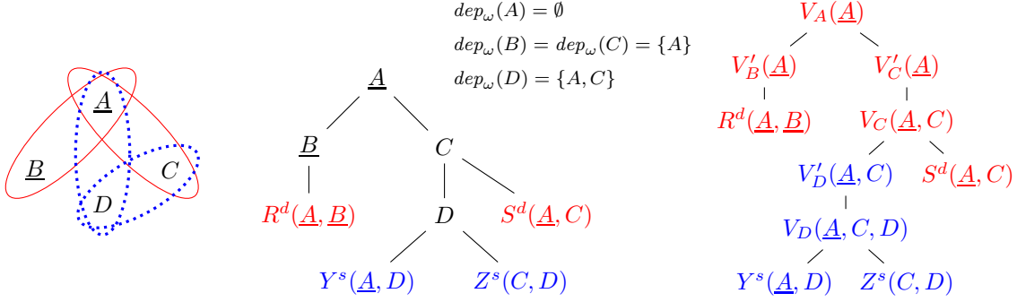
Figure 4: (left to right) The hypergraph of Q(A, B) = R^d(A, B), S^d(A, C), Y^s(A, D), Z^s(C, D) , a VO \omega for Q , and the view tree for Q constructed by the procedure \text{REWRITE}(\omega) from Figure 8. Dynamic views are in red, static views are in blue. The query Q has safe paths and the preprocessing width of 2, thus Q \in \mathcal{C}_{\text{poly}} .
