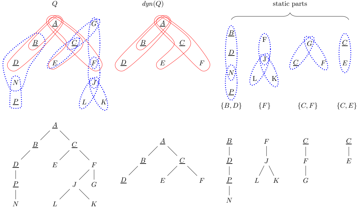
Figure 7: (top) Query Q , its dynamic sub-query dyn(Q) , and its static parts with the intersection sets. (bottom) Free-top VO for Q , free-top canonical VO for dyn(Q) , and free-top VOs with neck \mathbf{Y} for each static part with intersection set \mathbf{Y} . For simplicity, the atoms in the VOs are omitted.
