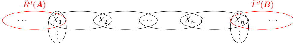
Figure 9: Illustration of a path in a query that does not have safe atom-to-atom paths.
