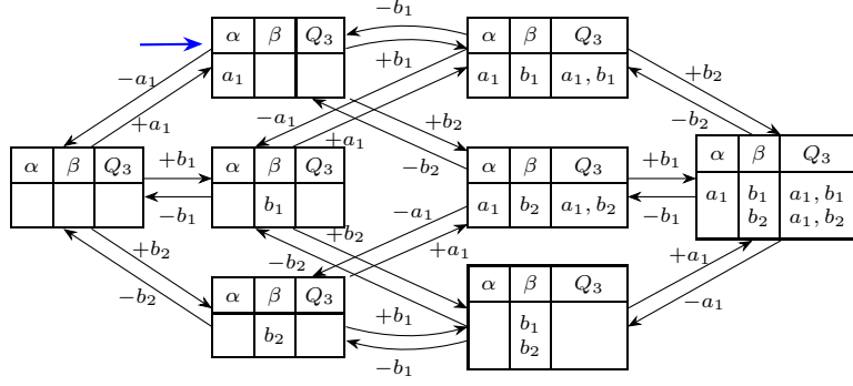
Figure 6: Left: Input database with two dynamic relations R^d(A) and T^d(B) and one static relation S^s(A, B) . Right: The transition system built from the input database and query Q_3 . Each state (box) corresponds to a pair of subsets \alpha and \beta of A -values and B -values in S^s (first two columns), and the corresponding materialized result of Q_3 if R^d and T^d contain the values in \alpha and \beta (third column). Each transition (arrow) corresponds to an insertion +a (deletion -a ) of an A -value a to (from) R^d or to insertion +b (deletion -b ) of a B -value b to (from) T^d . The initial state has \alpha = \{a_1\} and \beta = \emptyset (blue incoming arrow).
