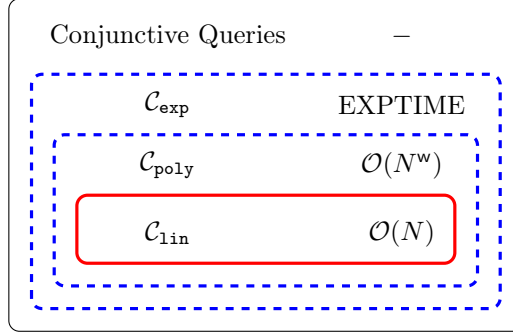
Figure 1: Classes \mathcal{C}_{\text{lin}} \subset \mathcal{C}_{\text{poly}} \subset \mathcal{C}_{\text{exp}} of tractable queries over static and dynamic relations and the corresponding preprocessing time (data complexity). N is the current database size and w is the preprocessing width. The solid (red) border around the class \mathcal{C}_{\text{lin}} states that there is a dichotomy between the queries inside and outside the class. The dashed (blue) border around a class states that no dichotomy is known for queries inside and outside the class.
