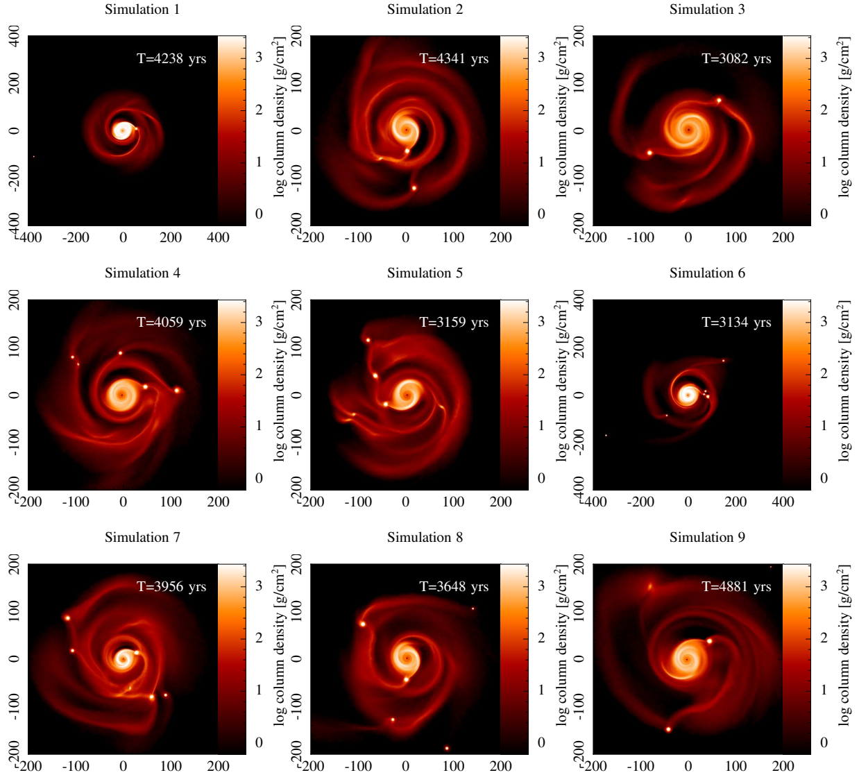
Figure 1. Column density plots of the final fragment configuration for all 9 simulations. Despite almost identical initial conditions, there are a variety of ultimate configurations, and a variety of times at which it becomes computationally unfeasible to continue the simulation using only hydrodynamics. Simulations 1 and 6 show an ejected clump at large radial separation, and the top left hand corner of simulation 9 shows a fragment forming just below the threshold detection of our algorithm.
