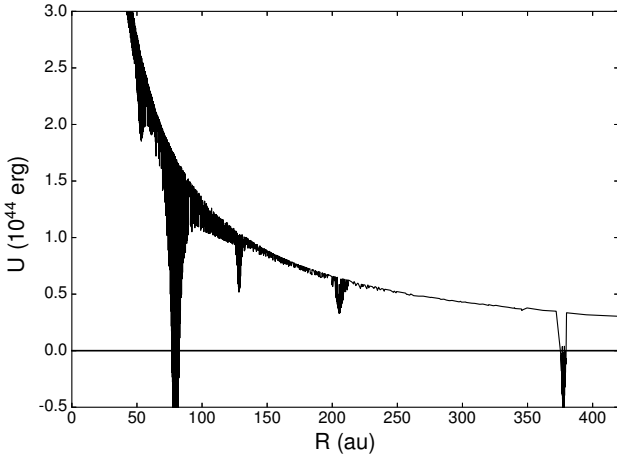
Figure 6. Radial profile of gravitational potential energy for the disc shown in Figure 1, simulation 6. Only two clumps, at r \sim 80 au and r \sim 375 au have a sufficiently deep potential well to be identified by our ordered potential search. The other three clumps, at r \sim 50 au, r \sim 125 au and r \sim 210 au are identified as belonging to the main body of the disc. Their detection in the density derivative search, but not in the ordered potential search, indicates that they would likely be tidally destroyed.
