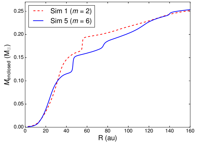
Figure 11. Disc mass enclosed as a function of radius for the final timesteps of simulation 1 (red dashed line) and simulation 5 (blue solid line). Since more mass is enclosed at shorter radii for simulation 1, more mass has been transported inwards in the disc, giving it a slightly steeper density profile.
