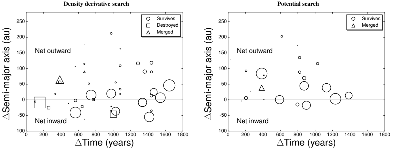
Figure 3. Plots showing total change in semi-major axis, for all clumps in all 9 simulations, plotted against the time between initial identification, and the either the end of the simulation, or the last timestep in which they are identified, if they are destroyed or merged. Larger markers correspond to more massive clumps. The left hand panel shows clumps as they are identified by our density derivative search method, and the right hand panel shows clumps as they are identified using our ordered potential search method. Circular markers indicate the clump survived the duration of the simulation, square markers indicate tidally destroyed clumps, and triangle markers indicate the clump was subsumed by another clump. The right hand panel shows that clumps that are ultimately destroyed are not detected by the ordered potential search. The left hand panel shows that \sim 20\% of fragments are ultimately tidally destroyed. There are no identical markers in both plots because the clumps are detected at different times in the simulation, and thus migrate different distances.
