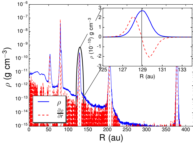
Figure 2. Our density derivative search method on the disc shown in Figure 1, simulation 6. The solid blue line shows the radial density profile of the disc, and the dashed red line shows the derivative of this with respect to r . The zoomed region demonstrates how the negative zero crossing of the derivative identifies one of the real density peaks.
