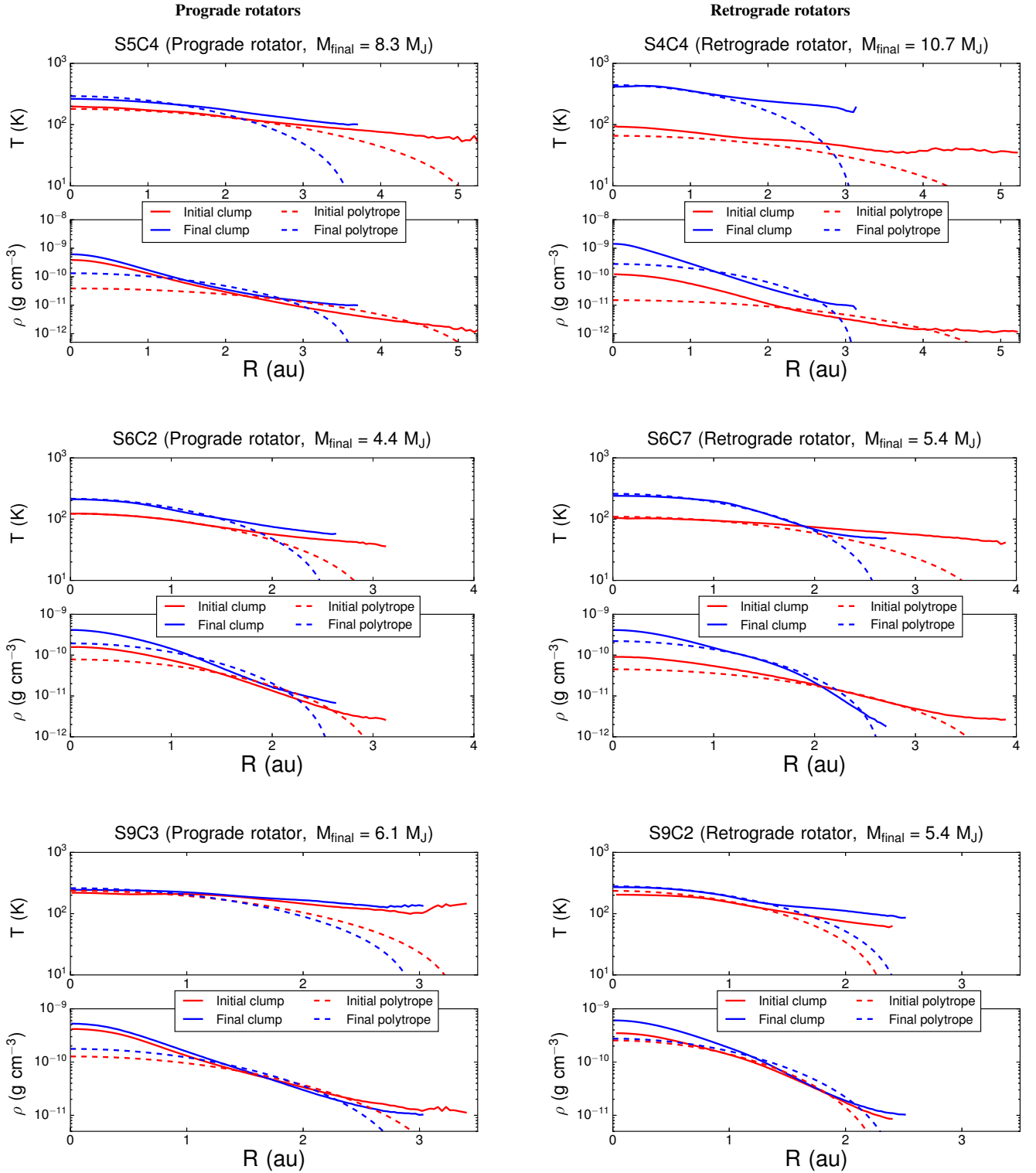
Figure 20. Radial density and temperature profiles for the initial and final state of 6 clumps. Red solid lines show initial clump profile, blue solid lines show final clump profile. For comparison, all clumps have initial and final n = 1.5 polytropic profiles plotted in initial and final states. The left column contains 3 clumps undergoing prograde rotation, and the right column shows 3 clumps undergoing retrograde rotation. In each row, the clumps are of comparable mass, and are intended to be compared, although bearing in mind that the clumps have had different evolutionary histories and their final masses are not identical. For most of the clumps, there is not much in their profiles that would mark them as a retro-rotating clump. The final inner and surface temperatures are similar, as is the shape of the density profile. Clump 4 in simulation 4 (top right panel) is somewhat the exception, with a large increase in both final inner density, inner temperature and surface temperature. Given the violent encounter it endured early in its history (shown in Figure 15), this may be unsurprising, but it is interesting to note that high surface temperatures may indicate a violent encounter in the past. In all cases, a polytrope of index n = 1.5 is a reasonable fit to the temperature profile, but consistently underestimates the inner density by around an order of magnitude.
