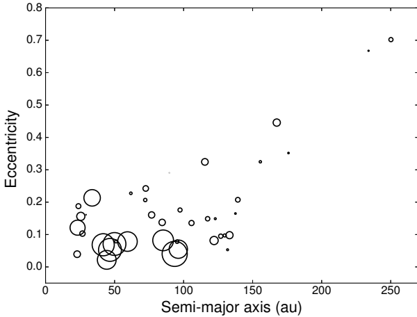
Figure 12. Final semi-major axis and eccentricity relation for our SPH clumps. Larger markers represent more massive clumps. The population synthesis model does not contain eccentricity data. We can see, for the most part, our clumps have a roughly linear relationship between eccentricity and semi-major axis, although there is a large amount of scatter.
