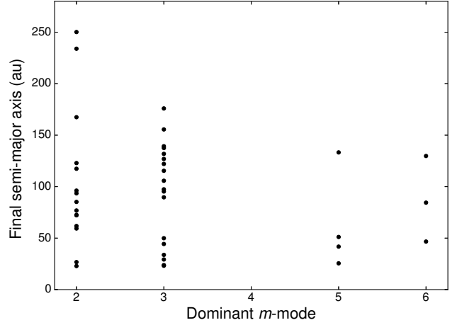
Figure 9. Final semi-major axis of all clumps in all simulations as detected by the density derivative search, as a function of the dominant m -mode in the disc. The largest semi-major axis require a 2 armed spiral, which is capable of exerting global torques. There appears to be a rough empirical relationship such that the maximum semi-major axis a_{\max} \propto 1/m , although this result is preliminary due to a small number of data points.
