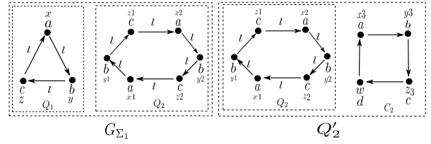
Figure 3: The satisfiability of GEDs
