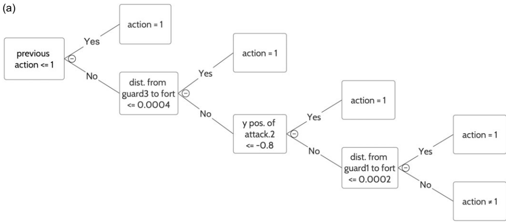
One FF tree in the ensemble for a guard in the FA domain.
