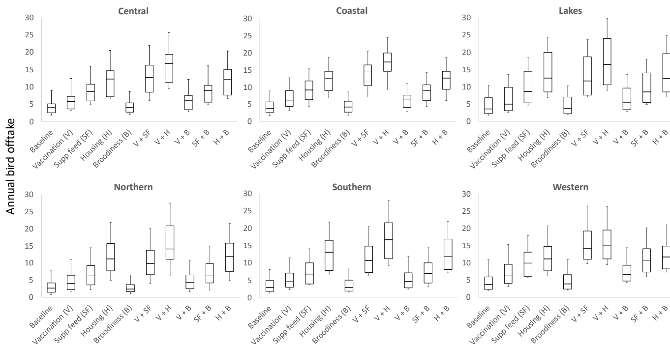
Annual bird offtake (consumed and sold) for the baseline and each intervention option across the six regions of Tanzania. Box plots are 10 th , 25 th , 50 th , 75 th and 90 th percentiles, reflecting the increase in flock size from small to large.
