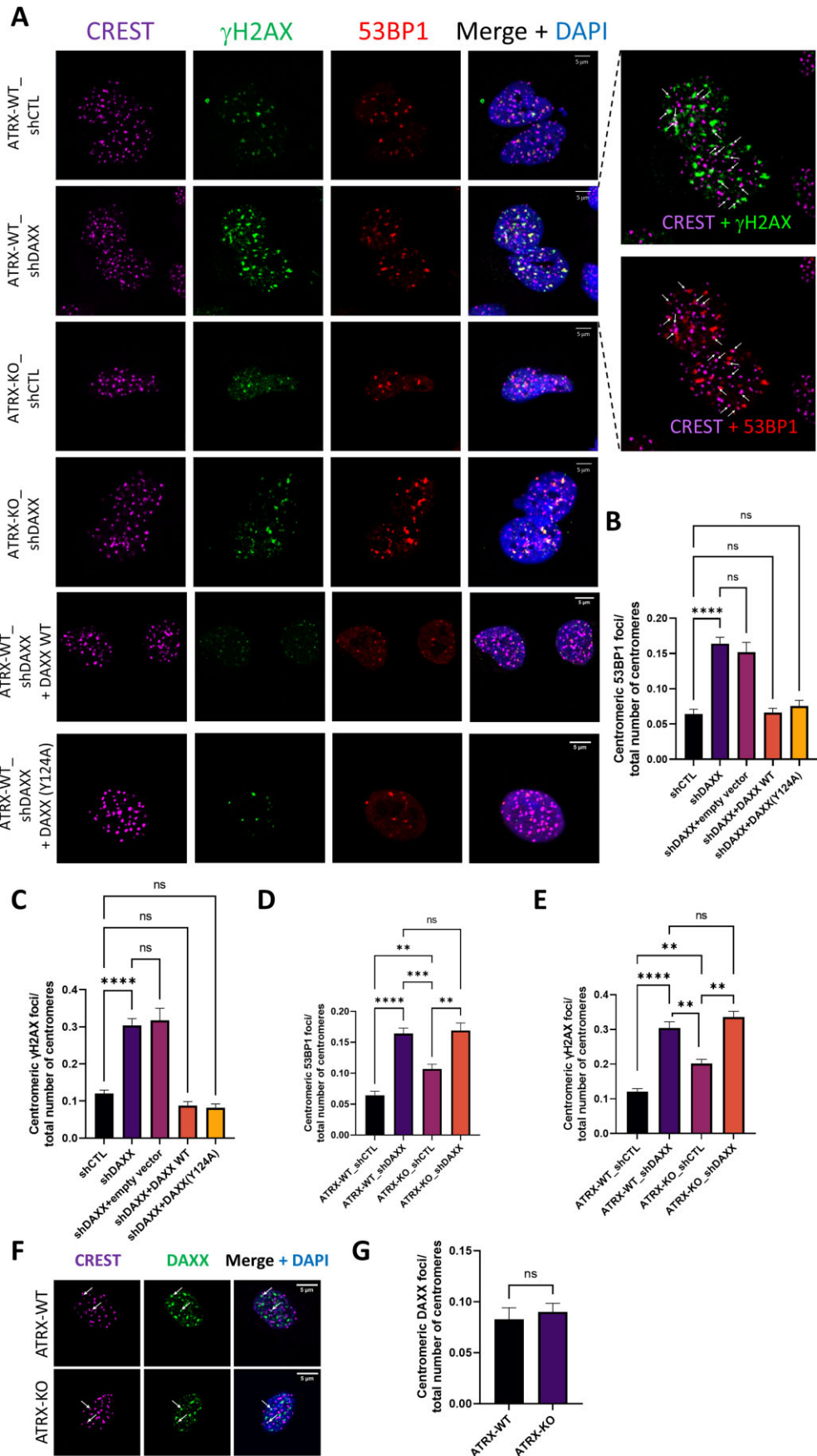
Figure 2. DAXX depletion increases spontaneous DNA damage at centromeres. (A) Representative IF images of CREST foci (centromeres, magenta), \gamma H2AX foci (green) and 53BP1 (red) in the indicated SF188 cell derivatives. White arrows in the rightmost panels point to representative CREST- \gamma H2AX
