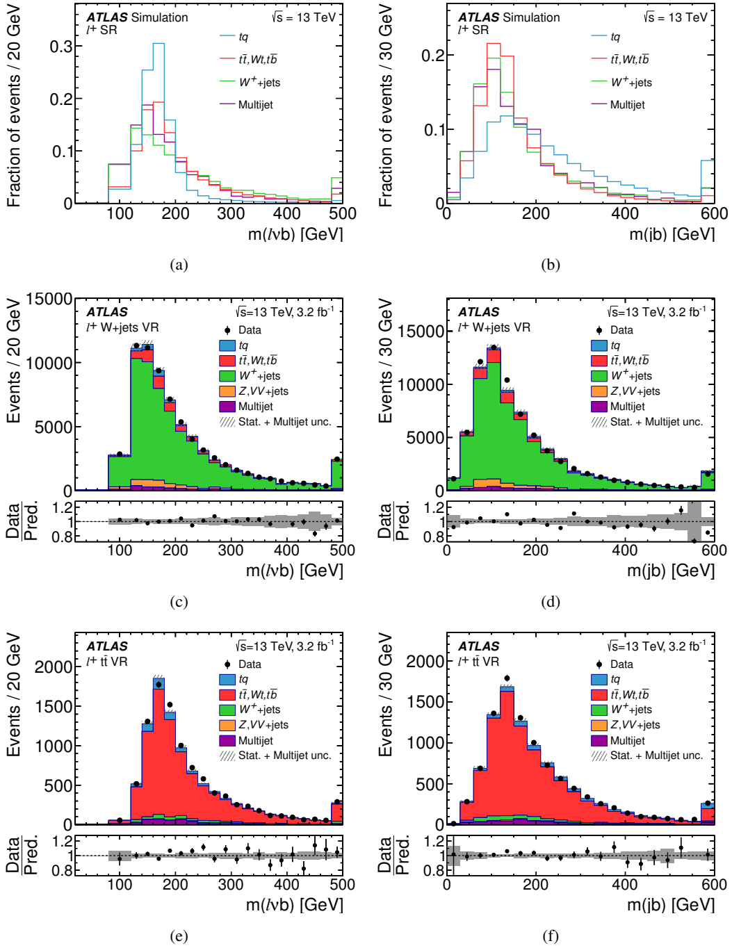
Figure 2. Distributions of the two most discriminating variables, (left) the reconstructed top-quark mass m(\ell vb) and (right) the invariant mass of the jet pair m(jb) , for the \ell^+ channel. In the t\bar{t} VR the b -jet used to calculate m(\ell vb) and m(jb) is the b -jet with the higher p_T . (a)-(b): signal and background distributions normalised to unit area. (c)-(f): observed distributions in the W +jets VR and the t\bar{t} VR compared to the model obtained from simulated events. The simulated distributions are normalised to match the number of observed events as described in the main text. The hatched and grey error bands represent the uncertainty in the number of multijet events and the uncertainty due to the size of the MC samples. The ratio of observed to predicted (Pred.) number of events in each bin is shown in the lower distributions. Events in the overflow are contained in the last bin.
