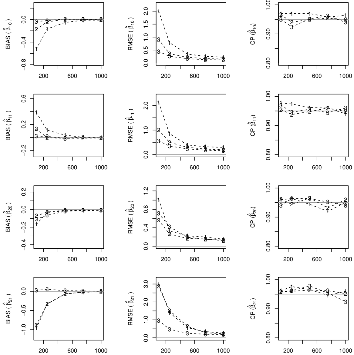
Figure 3: Bias, square root of mean squared error and coverage probability (CP) of the maximum likelihood estimation ( \hat{\beta}_{10}, \hat{\beta}_{11}, \hat{\beta}_{20}, \hat{\beta}_{21} ) of zero-inflated Weibull non-default rate regression model for simulated data under the three scenarios of parameters (the numbers 1, 2 and 3 on the graphs refer to the three scenarios), obtained from Monte Carlo simulations with 1000 replications and an increasing sample size ( n ).
