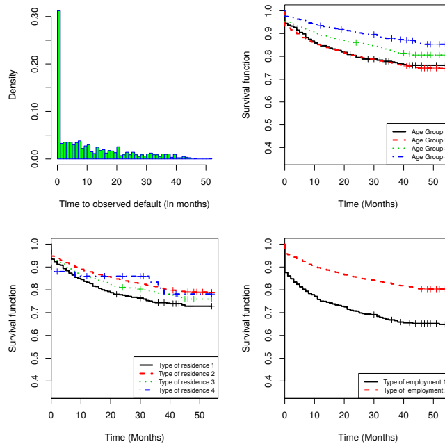
Figure 6: Brazilian bank loan portfolio data. The graphs at the top show histograms for the observed time-to-default variable of interest (left) and Kaplan-Meier survival curves stratified by age group (right). The graphs at the bottom show Kaplan-Meier survival curves stratified by type of residence (left) and Kaplan-Meier survival curves stratified by type of employment (right).
