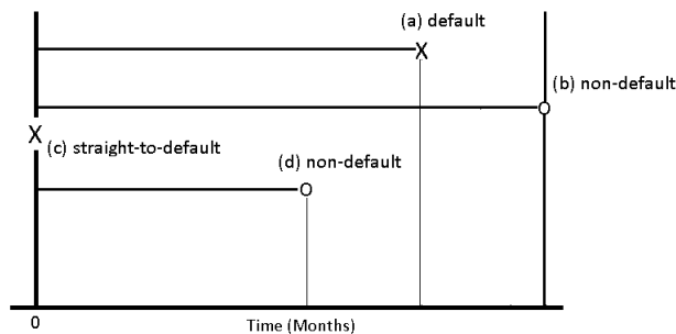
Figure 1: Loan survival time data.
