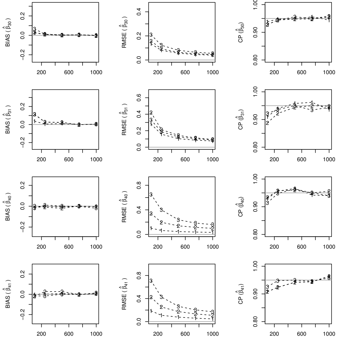
Figure 4: Bias, square root of mean squared error and coverage probability (CP) of the maximum likelihood estimation ( \hat{\beta}_{30}, \hat{\beta}_{31}, \hat{\beta}_{40}, \hat{\beta}_{41} ) of zero-inflated Weibull non-default rate regression model for simulated data under the three scenarios of parameters (the numbers 1, 2 and 3 on the graphs refer to the three scenarios), obtained from Monte Carlo simulations with 1000 replications and an increasing sample size ( n ).
