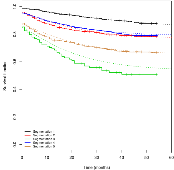
Figure 7: Brazilian bank loan portfolio. Kaplan-Meier survival curves stratified through the covariate selection given by the final model presented in Table 3 and the estimated survival curves (dotted lines)
