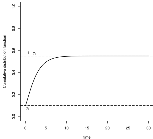
Figure 2: The CDF of the zero-inflated non-default rate model.
