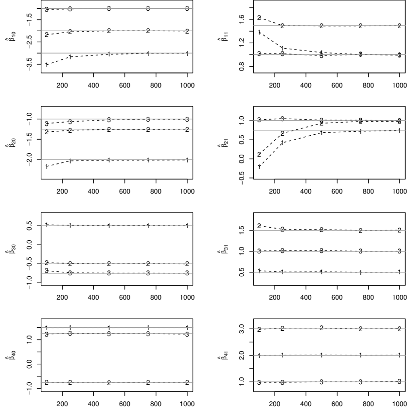
Figure 5: MLEA, maximum likelihood estimation on average of the parameters (\hat{\beta}_{10}, \hat{\beta}_{11}, \hat{\beta}_{20}, \hat{\beta}_{21}, \hat{\beta}_{30}, \hat{\beta}_{31}, \hat{\beta}_{40}, \hat{\beta}_{41}) of zero-inflated Weibull non-default rate regression model for simulated data under the three scenarios of parameters (the numbers 1, 2 and 3 on the graphs refer to the three scenarios), obtained from Monte Carlo simulations with 1000 replications and an increasing sample size ( n ).
