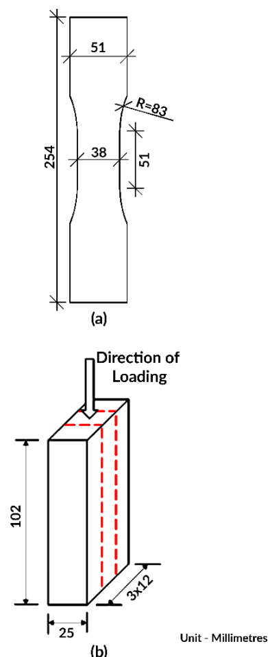
Figure 2 - Calcium Silicate: (a) Tensile coupon, (b) Compressive coupon
