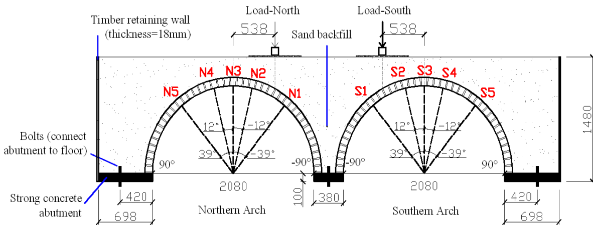
Figure 1: Schematic arch model (dimensions in mm)
