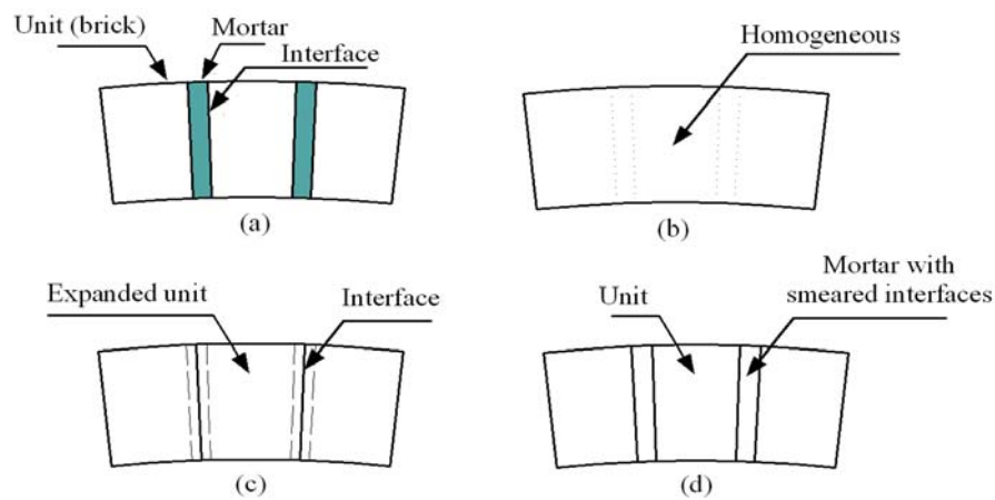
Figure 2: Modelling strategies for masonry arch: (a) local details of masonry work; (b) homogeneous model; (c) meso-interface model; (d) detailed solid model
