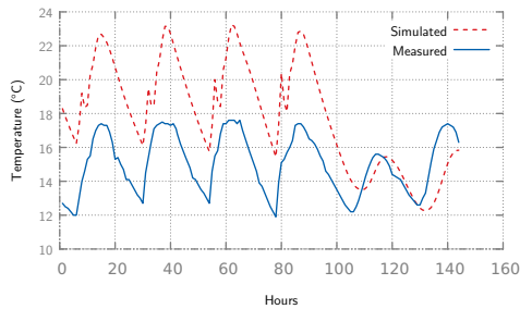
Figure 7. Temperature : March 20th-25th 2012 : Living Room, Setpoint 17.3°C [Calibrated Database values, 59mm wool external, 59mm wool internal].
