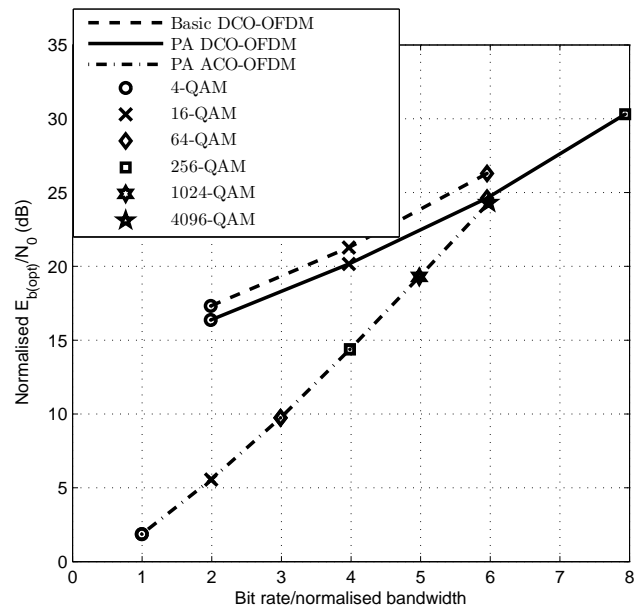
Fig. 7: E_{b(\text{opt})}/N_0 against bit rate/normalized bandwidth for basic DCO-OFDM, PA DCO-OFDM and ACO-OFDM signal with U = 5 , P = 5 , n_s = 127 , \text{BER} = 10^{-3} and [4, 16, 64, 256, 1024, 4096] -QAM.
