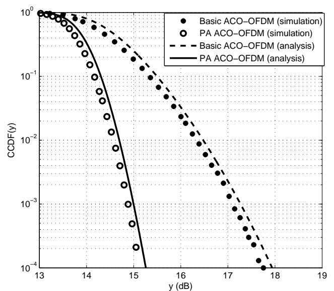
Fig. 3: CCDF plot of analytical and simulated basic and PA ACO-OFDM signal P = 5 , U = 5 , n_s = 127 and N = 508
