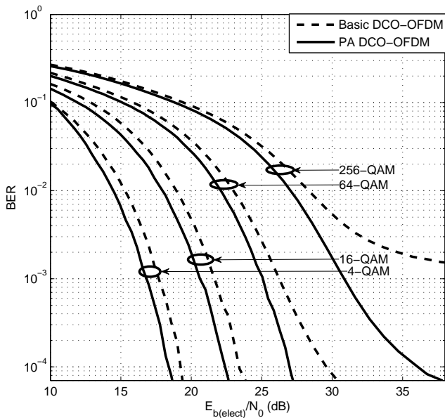
Fig. 6: BER performance for basic and PA DCO-OFDM signal with U = 5 , P = 5 , N = 256 , and [4, 16, 64, 256] -QAM
