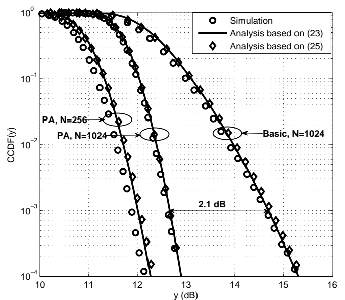
Fig. 2: CCDF plot for basic and PA O-OFDM signal using P = 5 , U = 5 , n_s = [127, 511] and N = [256, 1024] .
