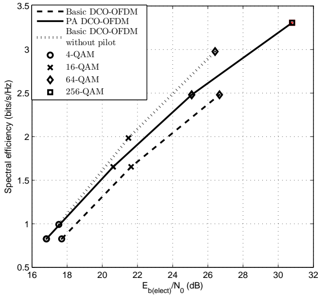
Fig. 8: Spectral efficiency against E_{b(\text{elect})}/N_0 for PA DCO-OFDM, basic DCO-OFDM with and without pilot symbol using U = 5 , P = 5 , N = 256 , \text{BER} = 10^{-3} , [4, 16, 64, 256]-QAM.
