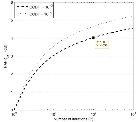
Fig. 4: PAPR reduction gain based on (41) at CCDF of 10^{-3} and 10^{-4} using U = 5 and N = 256 .
