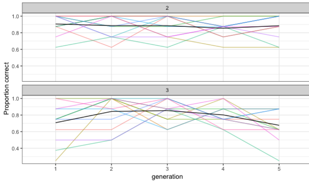
Figure a4: Experiment 2, comprehension accuracy by level, generation and number of objects (1-object entries are not included as these were trained to criterion). Colored lines are chains; the black line represents the mean across all chains.
