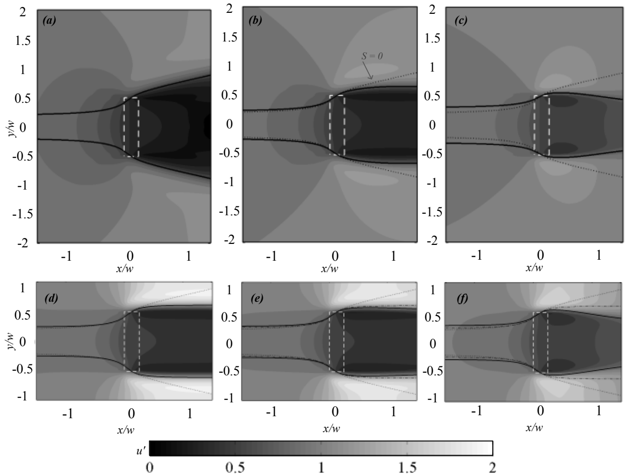
Figure 2. Contours of u' for (a) S = 0, B = 0.05 ; (b) S = 0.09, B = 0.05 ; (c) S = 0.5, B = 0.05 ; (d) S = 0, B = 0.5 ; (e) S = 0.09, B = 0.5 and (f) S = 0.5, B = 0.5 . Solid lines indicate streamlines bounding flow through the centre of the obstacle, dash-dot lines indicate the corresponding streamlines for S = 0 and the same blockage ratio, and dotted lines indicate the streamlines for S = 0, B = 0.05 . Dashed line represents the obstacle outline. A_R = 4, k = 12 .
