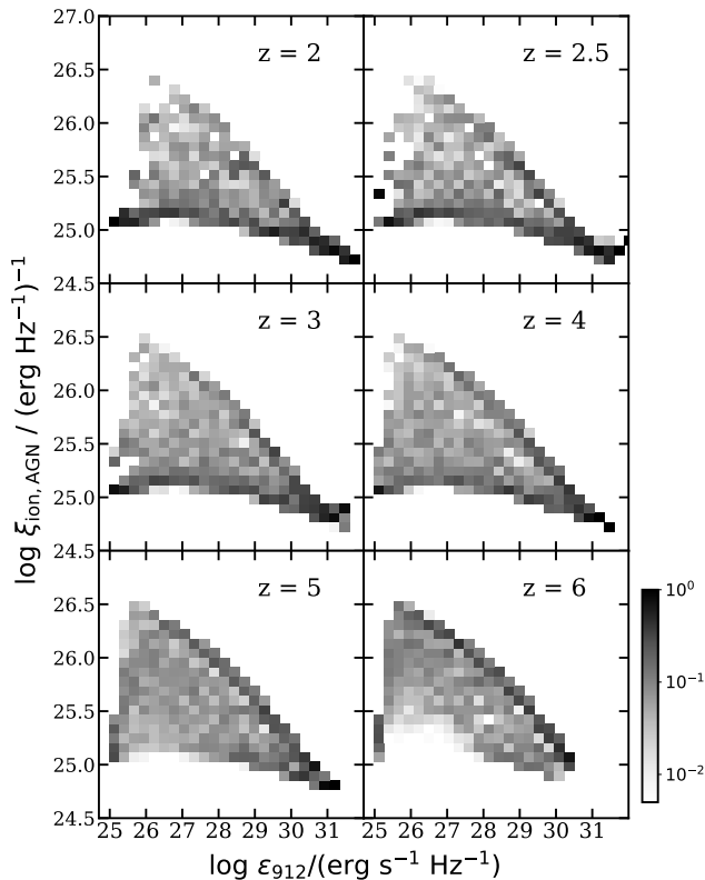
Figure 12. Conditional distributions of \xi_{\text{ion,AGN}} versus \epsilon_{912} between z = 2 to 6 , predicted by our fiducial model. The 2D histogram is colour-coded with the conditional number density per \text{Mpc}^3 of AGN in each bin, normalized to the sum of the number density in the corresponding (vertical) \epsilon_{912} bin.
