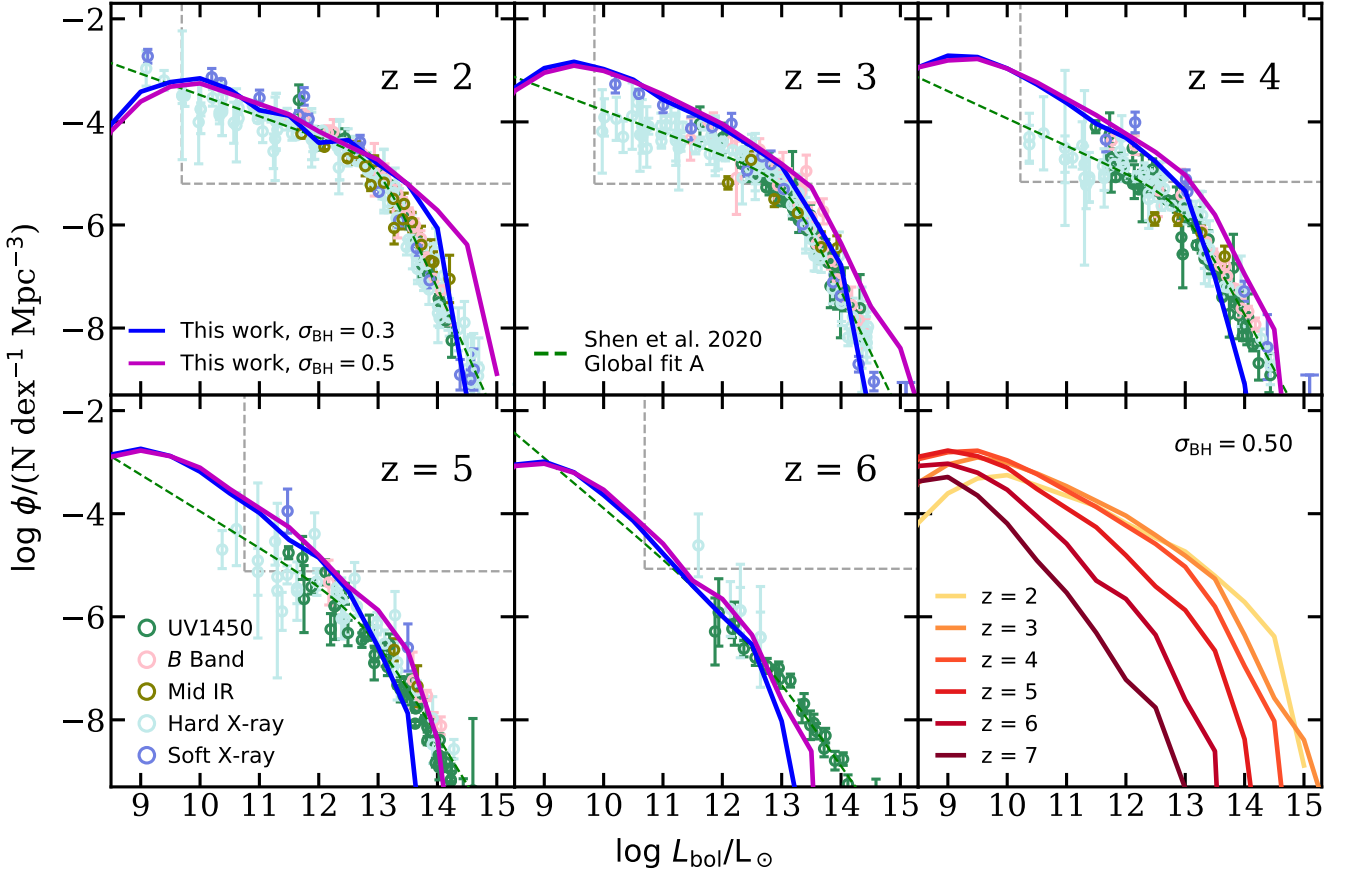
Figure 8. Predicted bolometric AGN luminosity functions and their evolution with redshift between z = 2 to 7 for our fiducial model ( \sigma_{\text{BH}} = 0.3 ; blue line) and adjusted model ( \sigma_{\text{BH}} = 0.5 ; purple line). These predictions are compared to multi-wavelength observational constraints compiled by Shen et al. (2020), which include bolometric corrections and dust and extinction corrections. We also show the fits to the bolometric LFs from S20 (global fit A; green dashed line). The grey dashed lines in each panel indicate the approximate range of objects that are expected to be detected in a typical JWST wide-field NIRCcam survey, where the vertical boundary loosely corresponds to the detection limit of m_{\text{F200W,lim}} = 28.60 and the horizontal line approximately represents where we expect to detect one object for a \sim 100 arcmin 2 survey area in a redshift slice of \Delta z = 0.5 . The last panel summarizes the predicted evolution of the bolometric LFs in the adjusted model. See text for full descriptions of individual elements included in this plot.
