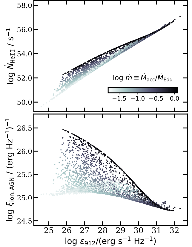
Figure 11. Distribution of \epsilon_{912} versus \dot{N}_{\text{ion,HeII}} ( top panel ) and \xi_{\text{ion,AGN}} ( bottom panel ) for our simulated AGN population, colour-coded by the Eddington-normalized accretion rate. Here we show AGN from at output at z = 3 ; however, this relation does not explicitly depend on redshift.
